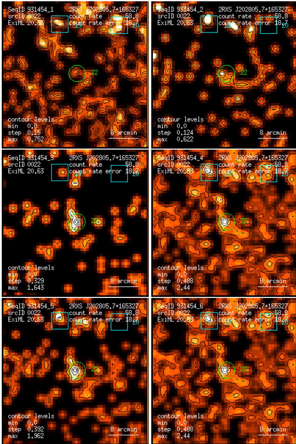
Figure 22: RASS 931454: detection 0022: band rate images, Gaussian filter: (1) PSPC channels 11 – 41, (2) 52 – 90, (3) 91 – 201, (4) 11 – 235, (5) 52 – 201, (6) 11 – 201. Broad band rates in counts/ks. Band rate contour levels in counts/ks/arcmin 2 .
