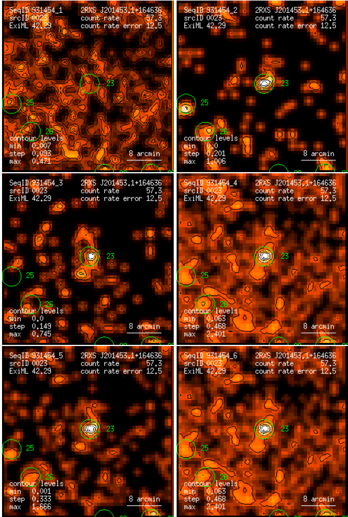
Figure 23: RASS 931454: detection 0023: band rate images, Gaussian filter: (1) PSPC channels 11 – 41, (2) 52 – 90, (3) 91 – 201, (4) 11 – 235, (5) 52 – 201, (6) 11 – 201. Broad band rates in counts/ks. Band rate contour levels in counts/ks/arcmin 2 .
