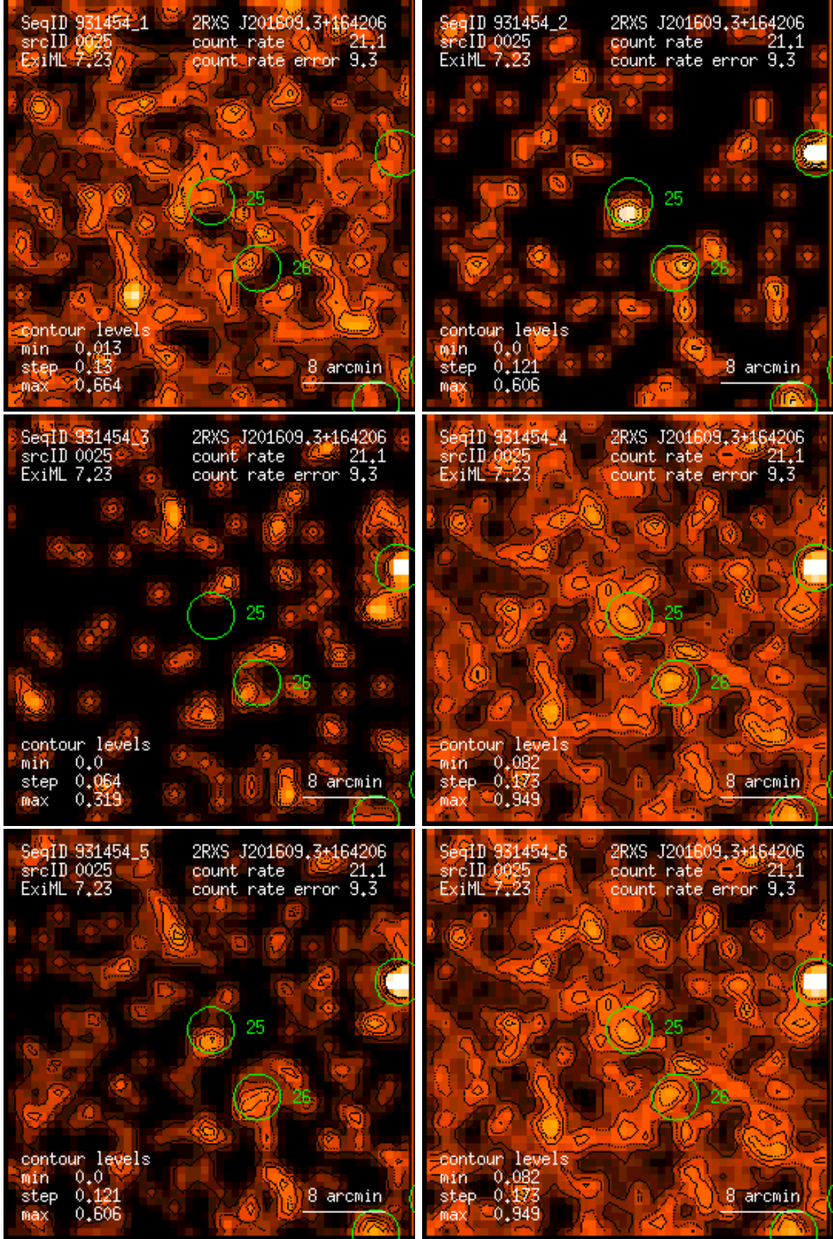
Figure 25: RASS 931454: detection 0025: band rate images, Gaussian filter: (1) PSPC channels 11 – 41, (2) 52 – 90, (3) 91 – 201, (4) 11 – 235, (5) 52 – 201, (6) 11 – 201. Broad band rates in counts/ks. Band rate contour levels in counts/ks/arcmin 2 .
