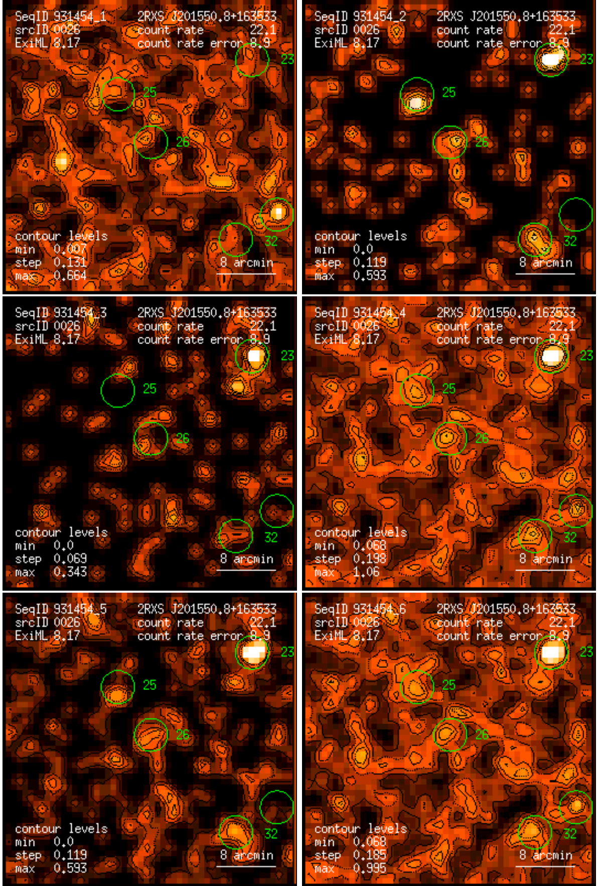
Figure 26: RASS 931454: detection 0026: band rate images, Gaussian filter: (1) PSPC channels 11 – 41, (2) 52 – 90, (3) 91 – 201, (4) 11 – 235, (5) 52 – 201, (6) 11 – 201. Broad band rates in counts/ks. Band rate contour levels in counts/ks/arcmin 2 .
