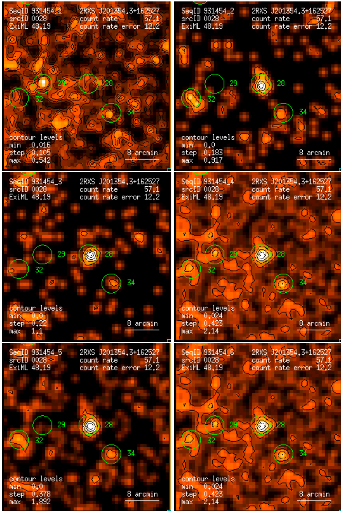
Figure 28: RASS 931454: detection 0028: band rate images, Gaussian filter: (1) PSPC channels 11 – 41, (2) 52 – 90, (3) 91 – 201, (4) 11 – 235, (5) 52 – 201, (6) 11 – 201. Broad band rates in counts/ks. Band rate contour levels in counts/ks/arcmin 2 .
