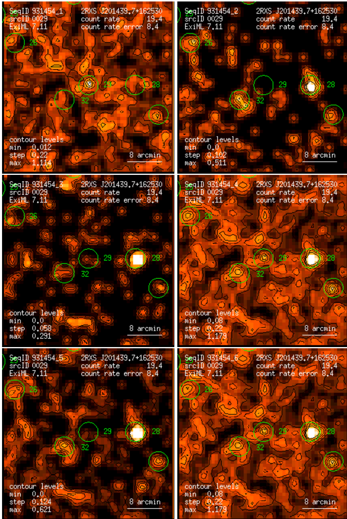
Figure 29: RASS 931454: detection 0029: band rate images, Gaussian filter: (1) PSPC channels 11 – 41, (2) 52 – 90, (3) 91 – 201, (4) 11 – 235, (5) 52 – 201, (6) 11 – 201. Broad band rates in counts/ks. Band rate contour levels in counts/ks/arcmin 2 .
