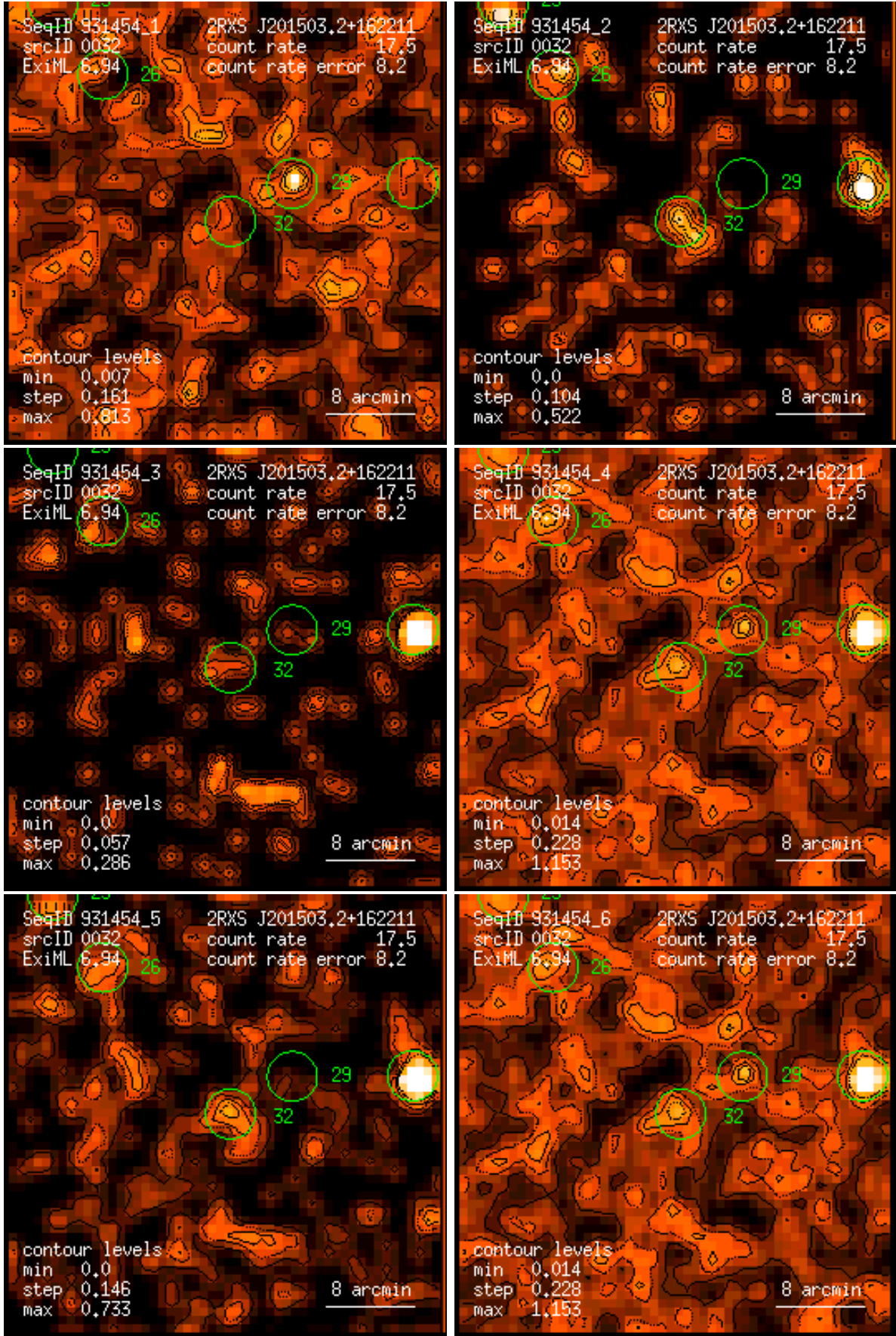
Figure 32: RASS 931454: detection 0032: band rate images, Gaussian filter: (1) PSPC channels 11 – 41, (2) 52 – 90, (3) 91 – 201, (4) 11 – 235, (5) 52 – 201, (6) 11 – 201. Broad band rates in counts/ks. Band rate contour levels in counts/ks/arcmin 2 .
