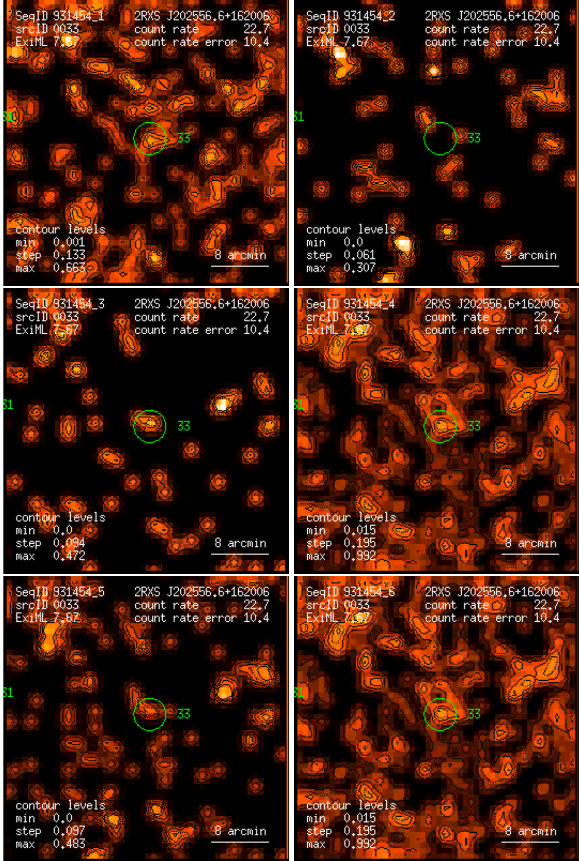
Figure 33: RASS 931454: detection 0033: band rate images, Gaussian filter: (1) PSPC channels 11 – 41, (2) 52 – 90, (3) 91 – 201, (4) 11 – 235, (5) 52 – 201, (6) 11 – 201. Broad band rates in counts/ks. Band rate contour levels in counts/ks/arcmin 2 .
