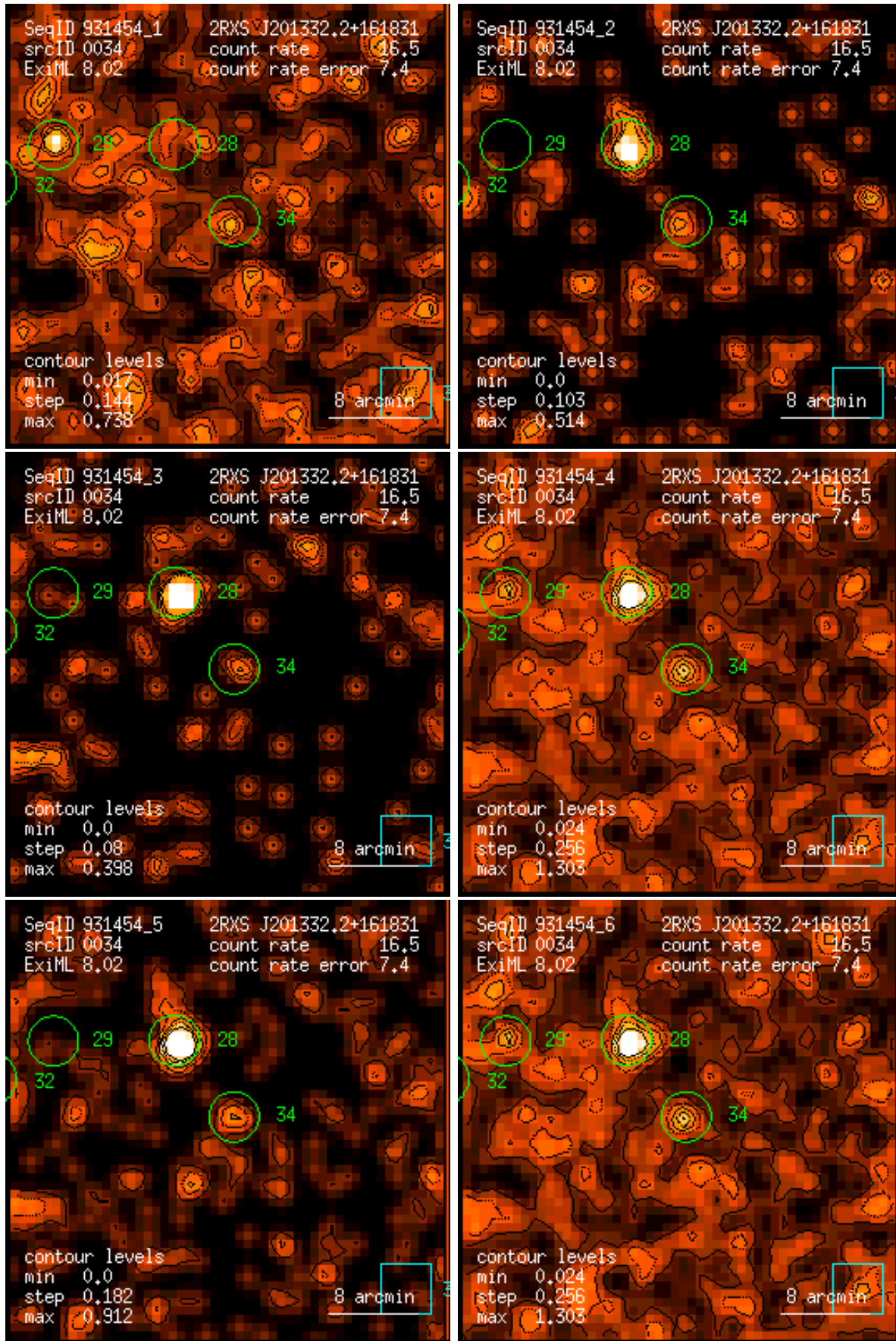
Figure 34: RASS 931454: detection 0034: band rate images, Gaussian filter: (1) PSPC channels 11 – 41, (2) 52 – 90, (3) 91 – 201, (4) 11 – 235, (5) 52 – 201, (6) 11 – 201. Broad band rates in counts/ks. Band rate contour levels in counts/ks/arcmin 2 .
