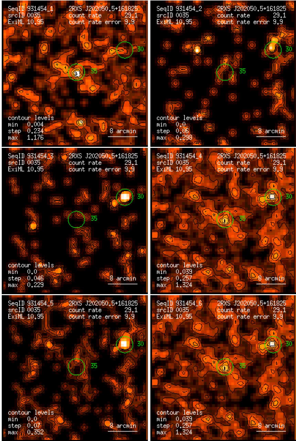
Figure 35: RASS 931454: detection 0035: band rate images, Gaussian filter: (1) PSPC channels 11 – 41, (2) 52 – 90, (3) 91 – 201, (4) 11 – 235, (5) 52 – 201, (6) 11 – 201. Broad band rates in counts/ks. Band rate contour levels in counts/ks/arcmin 2 .
