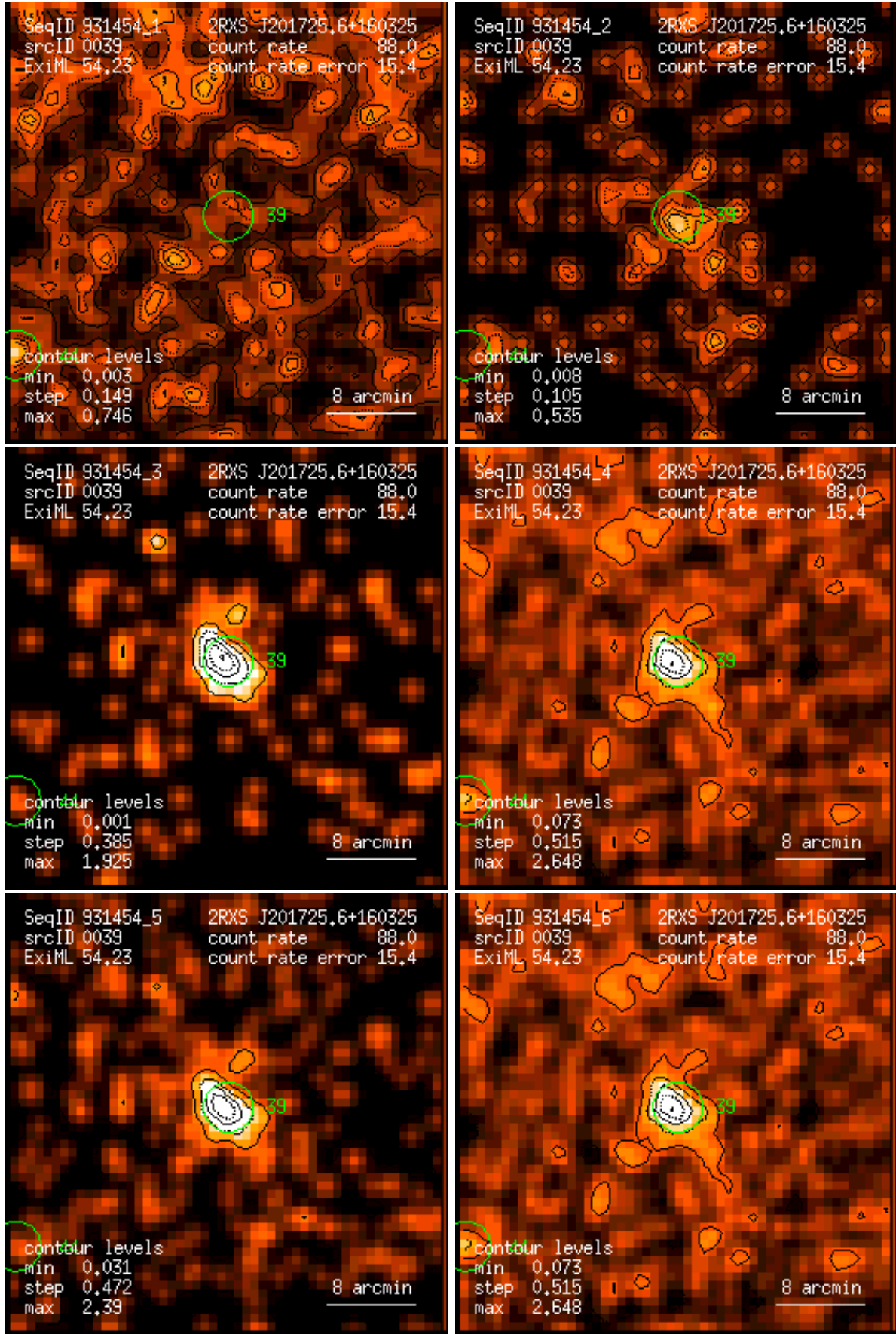
Figure 39: RASS 931454: detection 0039: band rate images, Gaussian filter: (1) PSPC channels 11 – 41, (2) 52 – 90, (3) 91 – 201, (4) 11 – 235, (5) 52 – 201, (6) 11 – 201. Broad band rates in counts/ks. Band rate contour levels in counts/ks/arcmin 2 .
