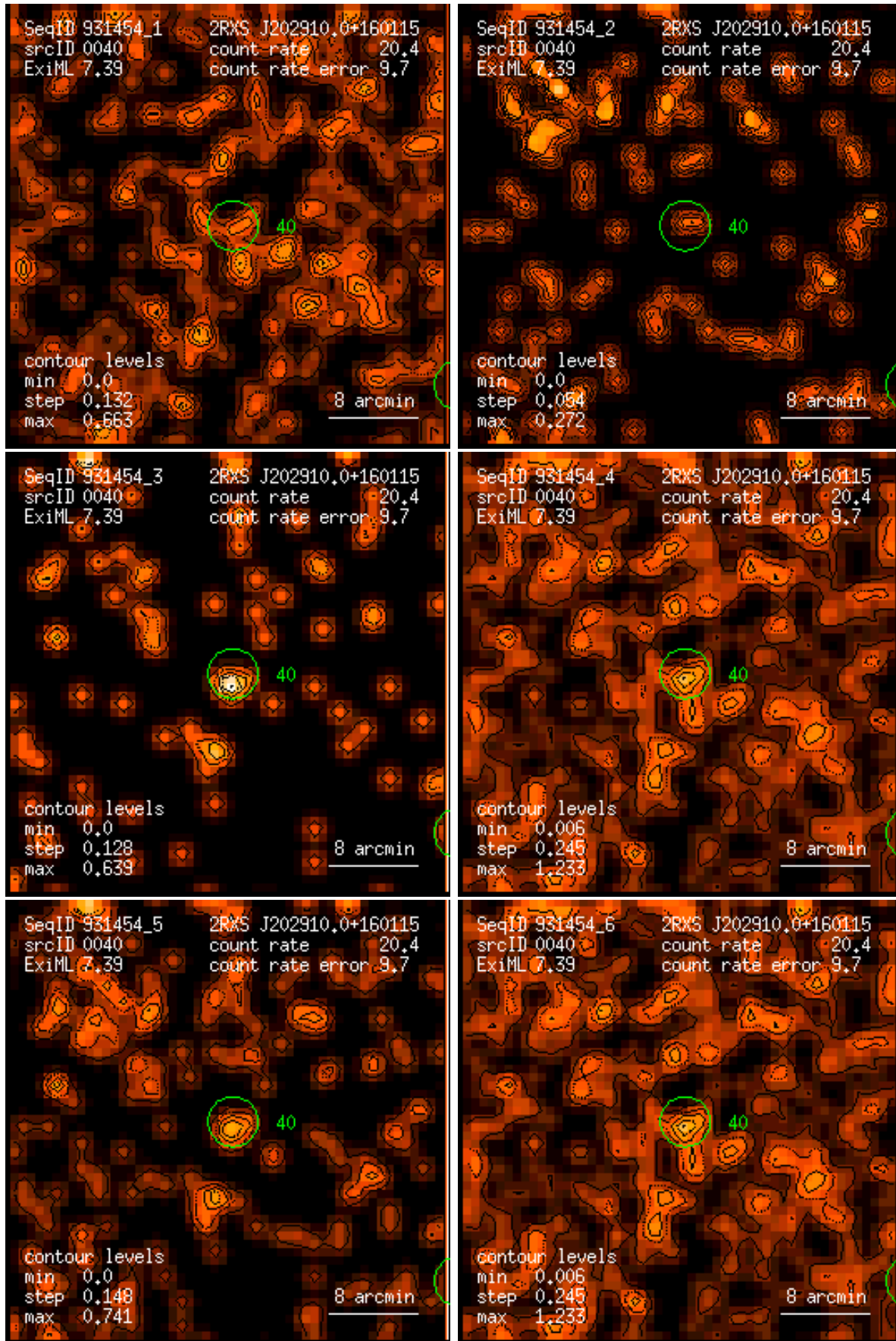
Figure 40: RASS 931454: detection 0040: band rate images, Gaussian filter: (1) PSPC channels 11 – 41, (2) 52 – 90, (3) 91 – 201, (4) 11 – 235, (5) 52 – 201, (6) 11 – 201. Broad band rates in counts/ks. Band rate contour levels in counts/ks/arcmin 2 .
