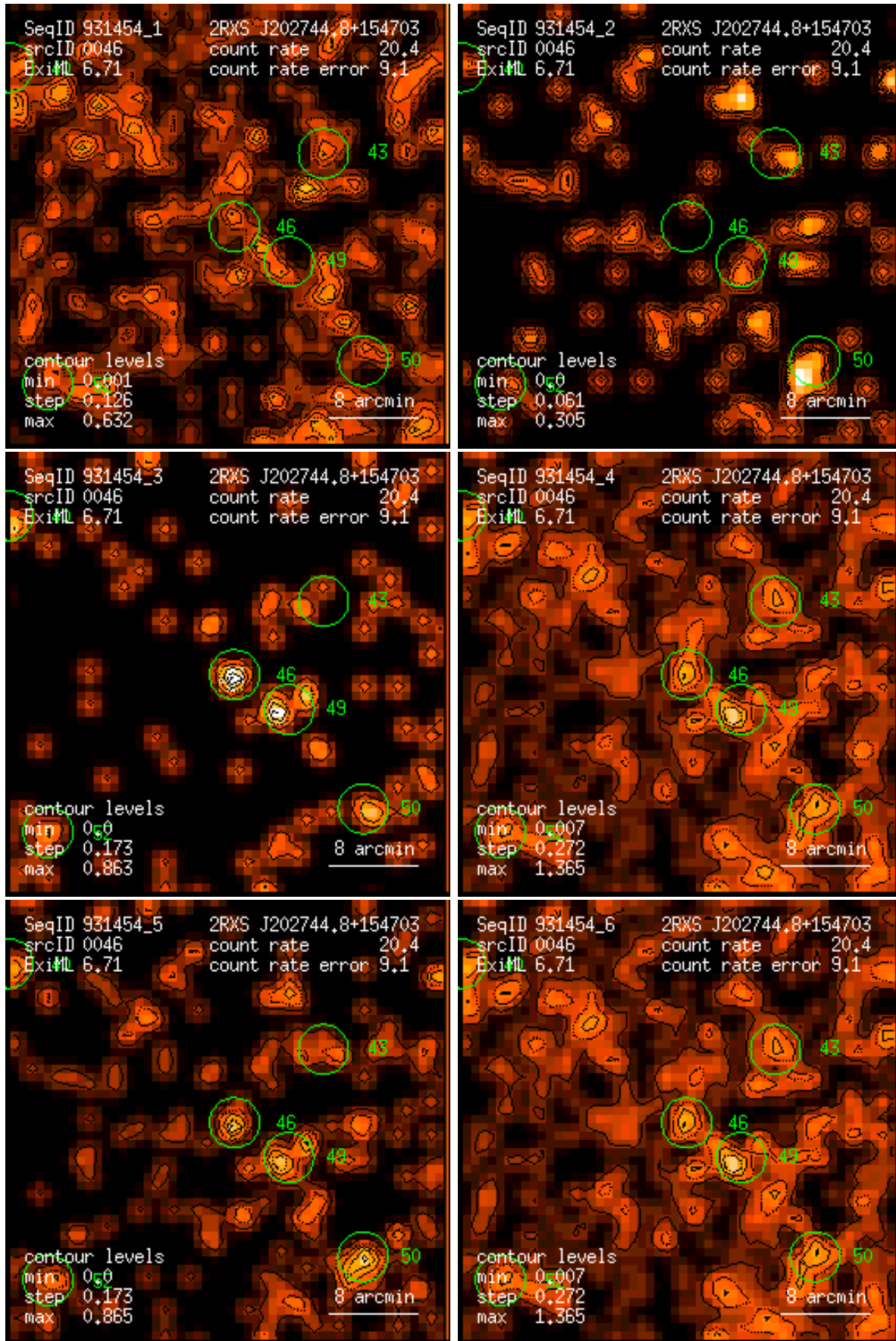
Figure 46: RASS 931454: detection 0046: band rate images, Gaussian filter: (1) PSPC channels 11 – 41, (2) 52 – 90, (3) 91 – 201, (4) 11 – 235, (5) 52 – 201, (6) 11 – 201. Broad band rates in counts/ks. Band rate contour levels in counts/ks/arcmin 2 .
