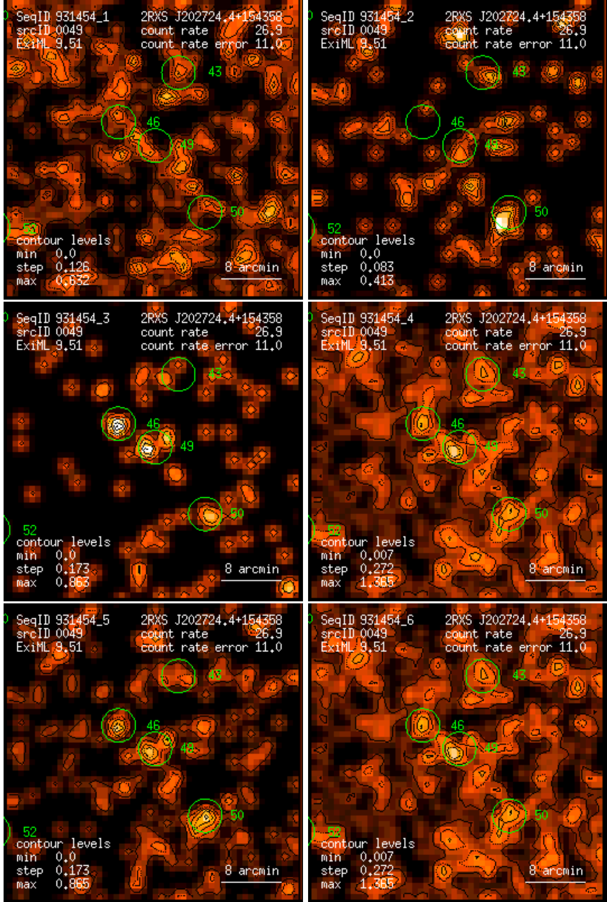
Figure 49: RASS 931454: detection 0049: band rate images, Gaussian filter: (1) PSPC channels 11 – 41, (2) 52 – 90, (3) 91 – 201, (4) 11 – 235, (5) 52 – 201, (6) 11 – 201. Broad band rates in counts/ks. Band rate contour levels in counts/ks/arcmin 2 .
