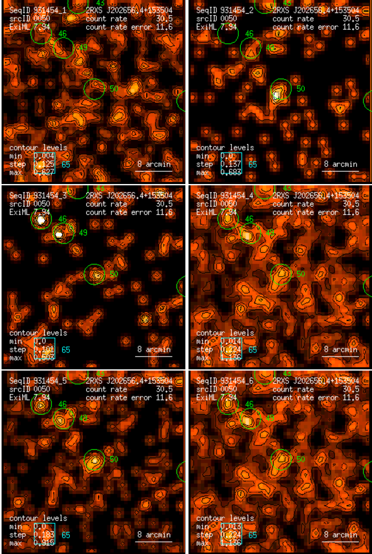
Figure 50: RASS 931454: detection 0050: band rate images, Gaussian filter: (1) PSPC channels 11 – 41, (2) 52 – 90, (3) 91 – 201, (4) 11 – 235, (5) 52 – 201, (6) 11 – 201. Broad band rates in counts/ks. Band rate contour levels in counts/ks/arcmin 2 .
