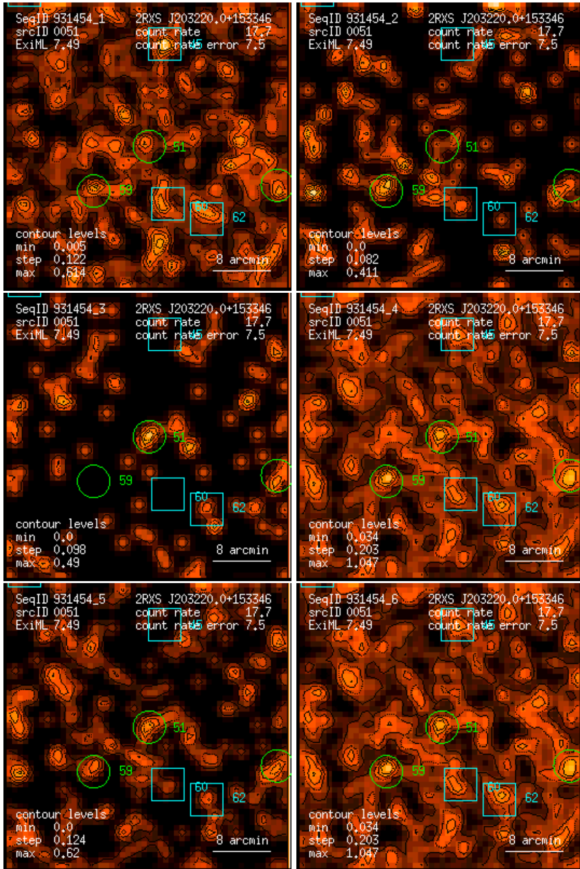
Figure 51: RASS 931454: detection 0051: band rate images, Gaussian filter: (1) PSPC channels 11 – 41, (2) 52 – 90, (3) 91 – 201, (4) 11 – 235, (5) 52 – 201, (6) 11 – 201. Broad band rates in counts/ks. Band rate contour levels in counts/ks/arcmin 2 .
