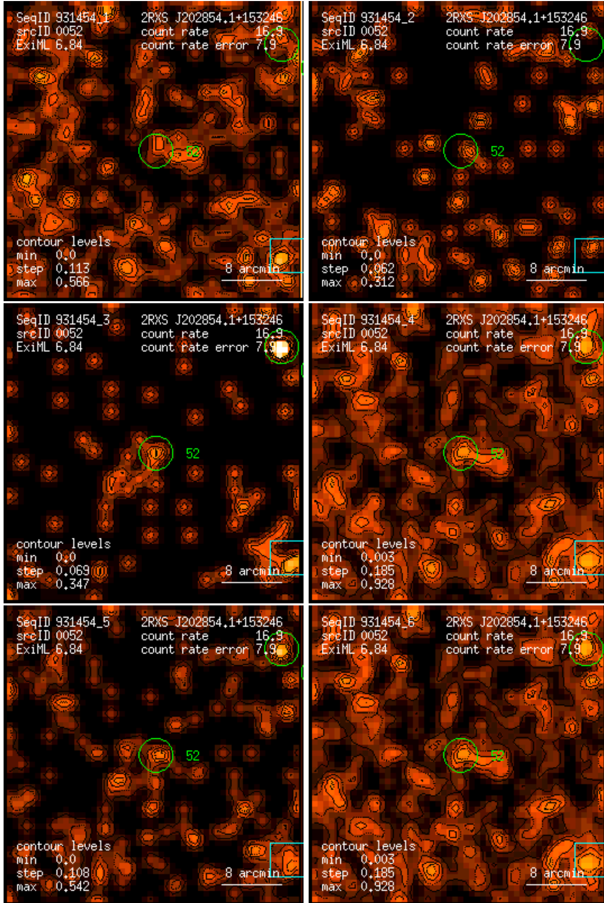
Figure 52: RASS 931454: detection 0052: band rate images, Gaussian filter: (1) PSPC channels 11 – 41, (2) 52 – 90, (3) 91 – 201, (4) 11 – 235, (5) 52 – 201, (6) 11 – 201. Broad band rates in counts/ks. Band rate contour levels in counts/ks/arcmin 2 .
