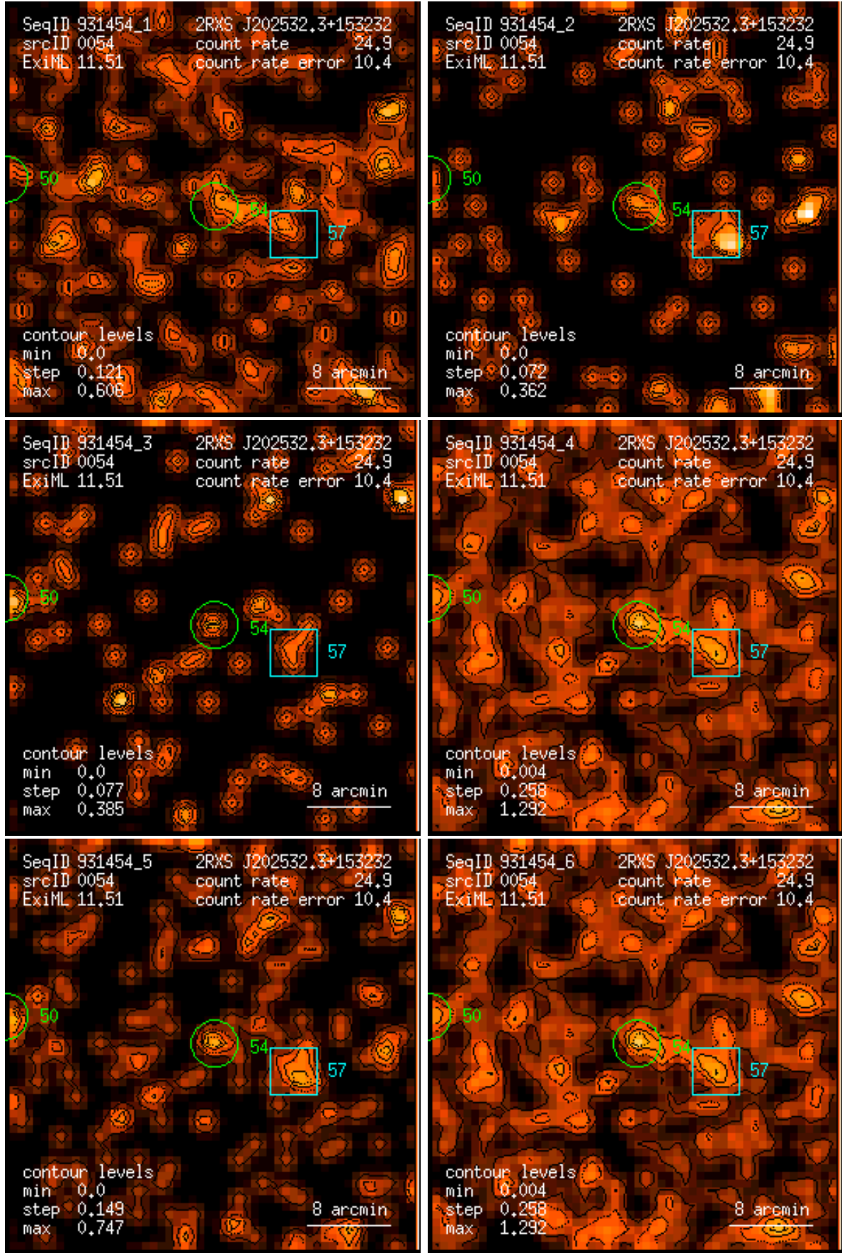
Figure 54: RASS 931454: detection 0054: band rate images, Gaussian filter: (1) PSPC channels 11 – 41, (2) 52 – 90, (3) 91 – 201, (4) 11 – 235, (5) 52 – 201, (6) 11 – 201. Broad band rates in counts/ks. Band rate contour levels in counts/ks/arcmin 2 .
