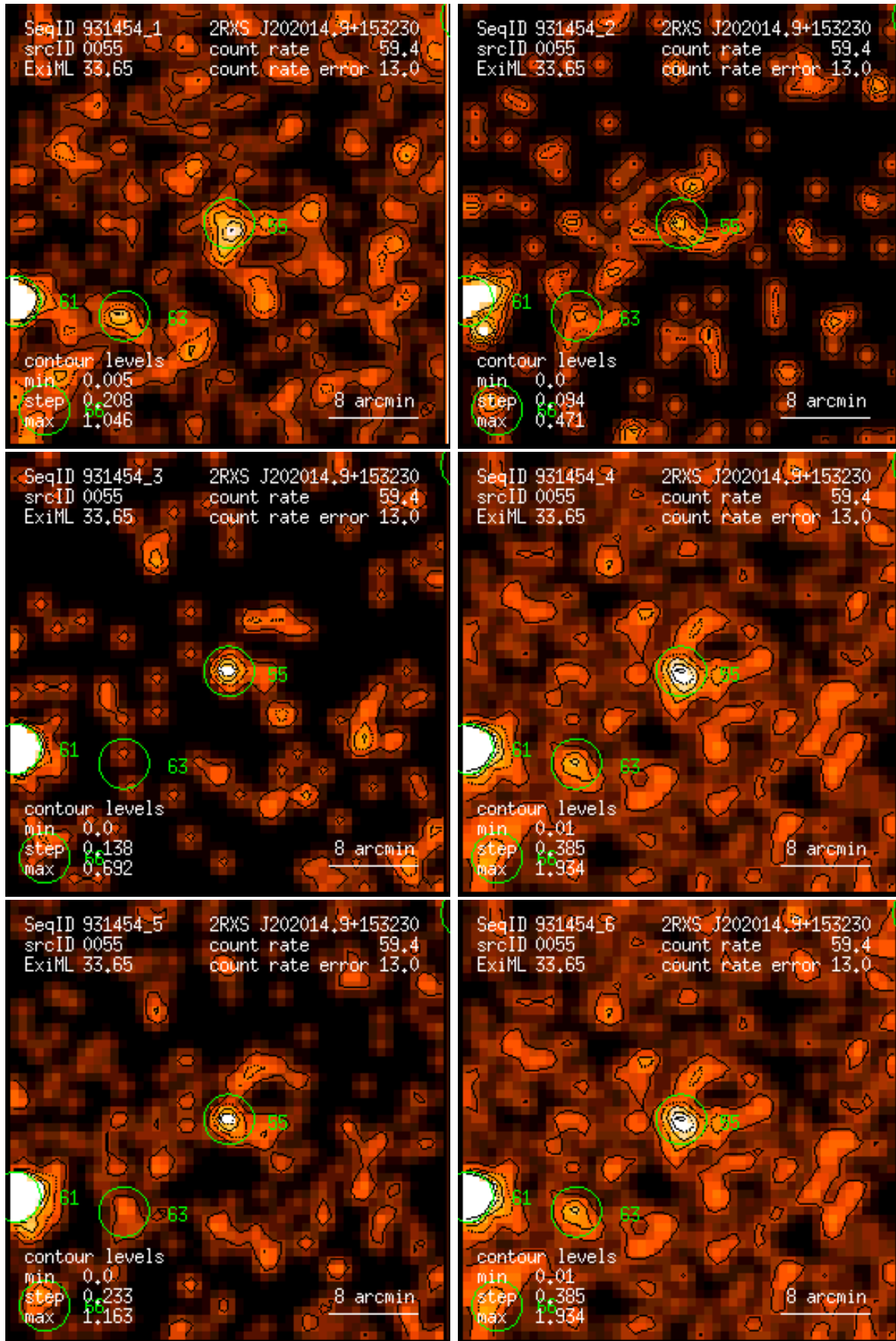
Figure 55: RASS 931454: detection 0055: band rate images, Gaussian filter: (1) PSPC channels 11 – 41, (2) 52 – 90, (3) 91 – 201, (4) 11 – 235, (5) 52 – 201, (6) 11 – 201. Broad band rates in counts/ks. Band rate contour levels in counts/ks/arcmin 2 .
