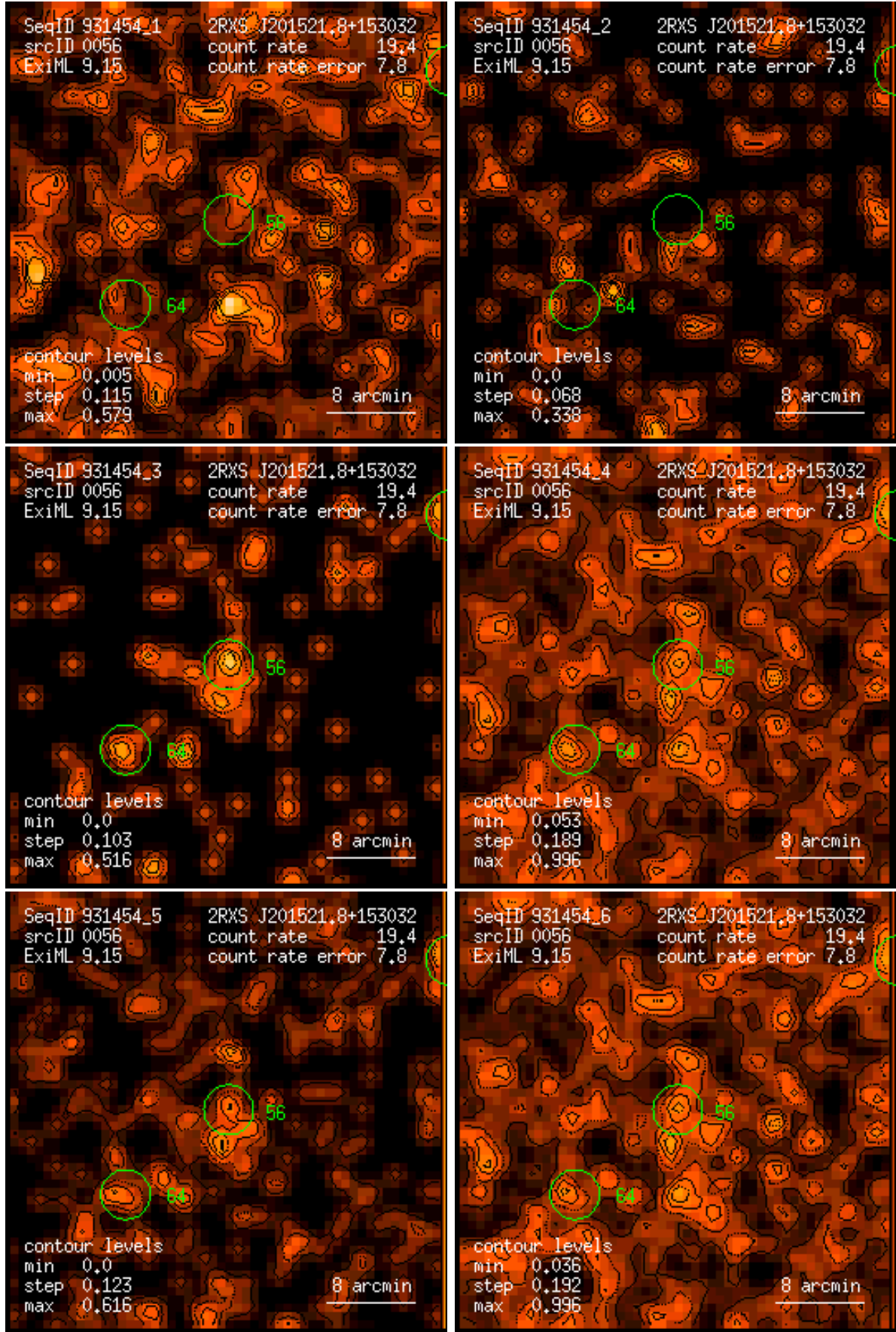
Figure 56: RASS 931454: detection 0056: band rate images, Gaussian filter: (1) PSPC channels 11 – 41, (2) 52 – 90, (3) 91 – 201, (4) 11 – 235, (5) 52 – 201, (6) 11 – 201. Broad band rates in counts/ks. Band rate contour levels in counts/ks/arcmin 2 .
