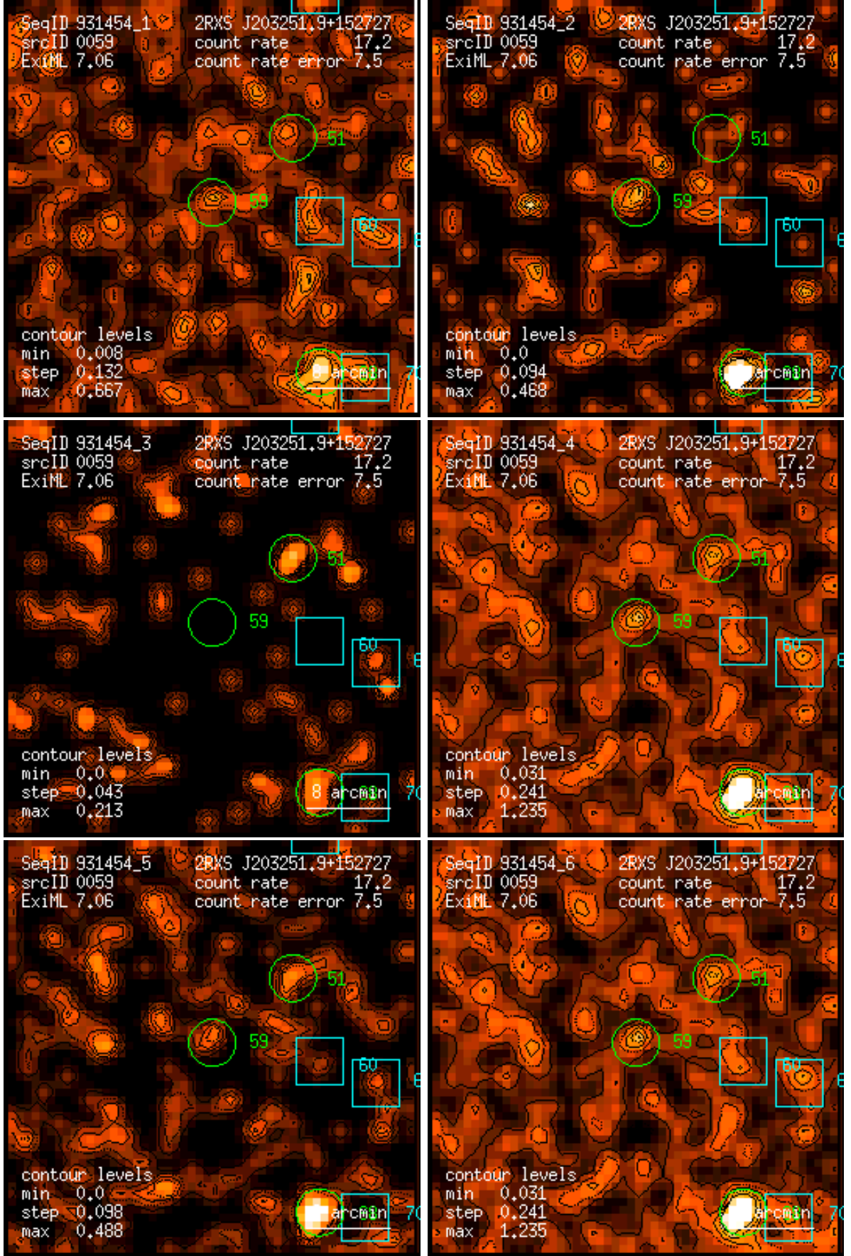
Figure 59: RASS 931454: detection 0059: band rate images, Gaussian filter: (1) PSPC channels 11 – 41, (2) 52 – 90, (3) 91 – 201, (4) 11 – 235, (5) 52 – 201, (6) 11 – 201. Broad band rates in counts/ks. Band rate contour levels in counts/ks/arcmin 2 .
