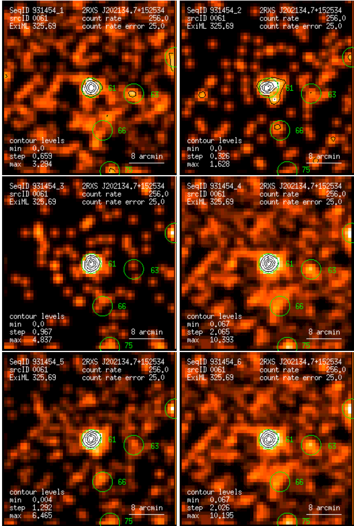
Figure 61: RASS 931454: detection 0061: band rate images, Gaussian filter: (1) PSPC channels 11 – 41, (2) 52 – 90, (3) 91 – 201, (4) 11 – 235, (5) 52 – 201, (6) 11 – 201. Broad band rates in counts/ks. Band rate contour levels in counts/ks/arcmin 2 .
