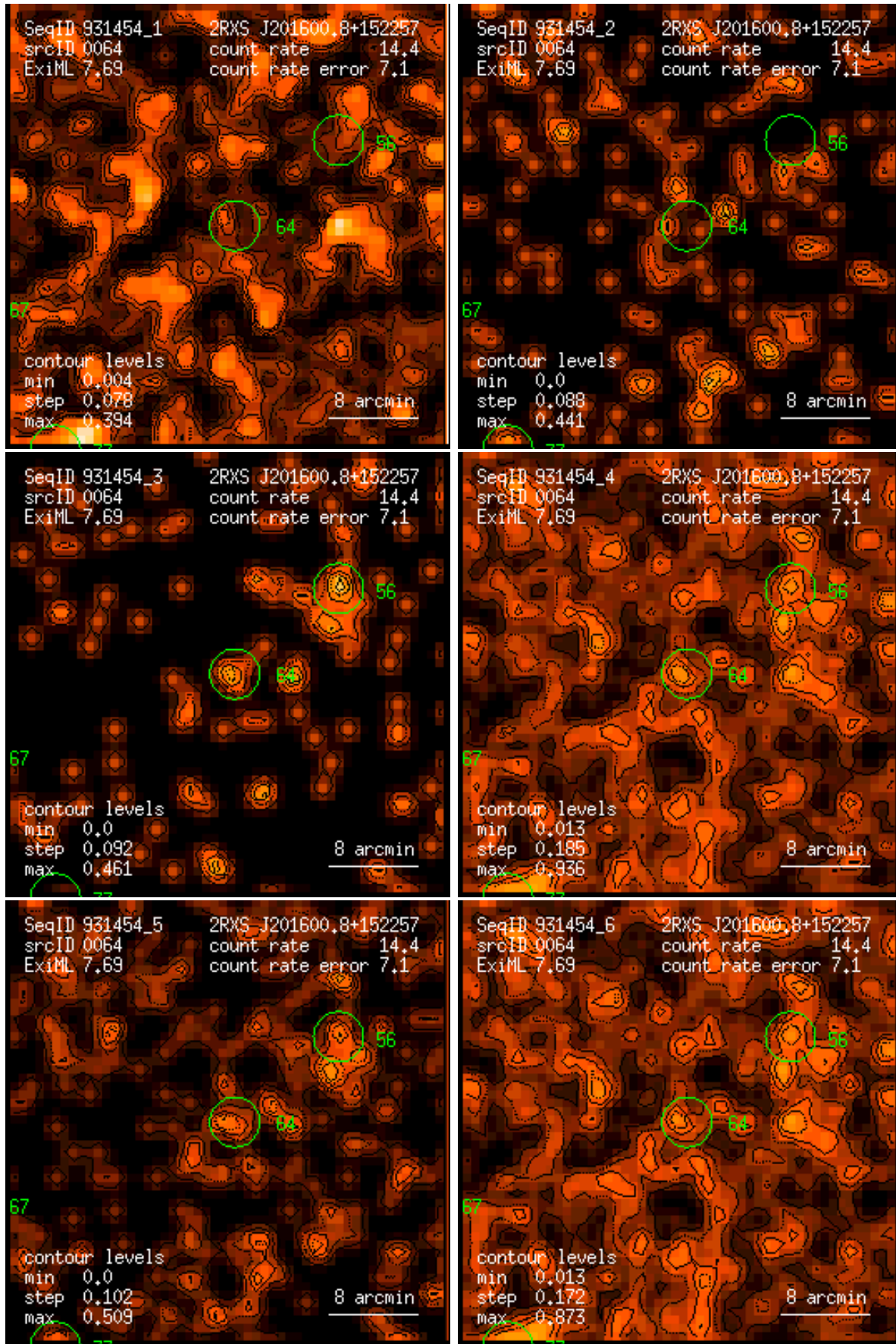
Figure 64: RASS 931454: detection 0064: band rate images, Gaussian filter: (1) PSPC channels 11 – 41, (2) 52 – 90, (3) 91 – 201, (4) 11 – 235, (5) 52 – 201, (6) 11 – 201. Broad band rates in counts/ks. Band rate contour levels in counts/ks/arcmin 2 .
