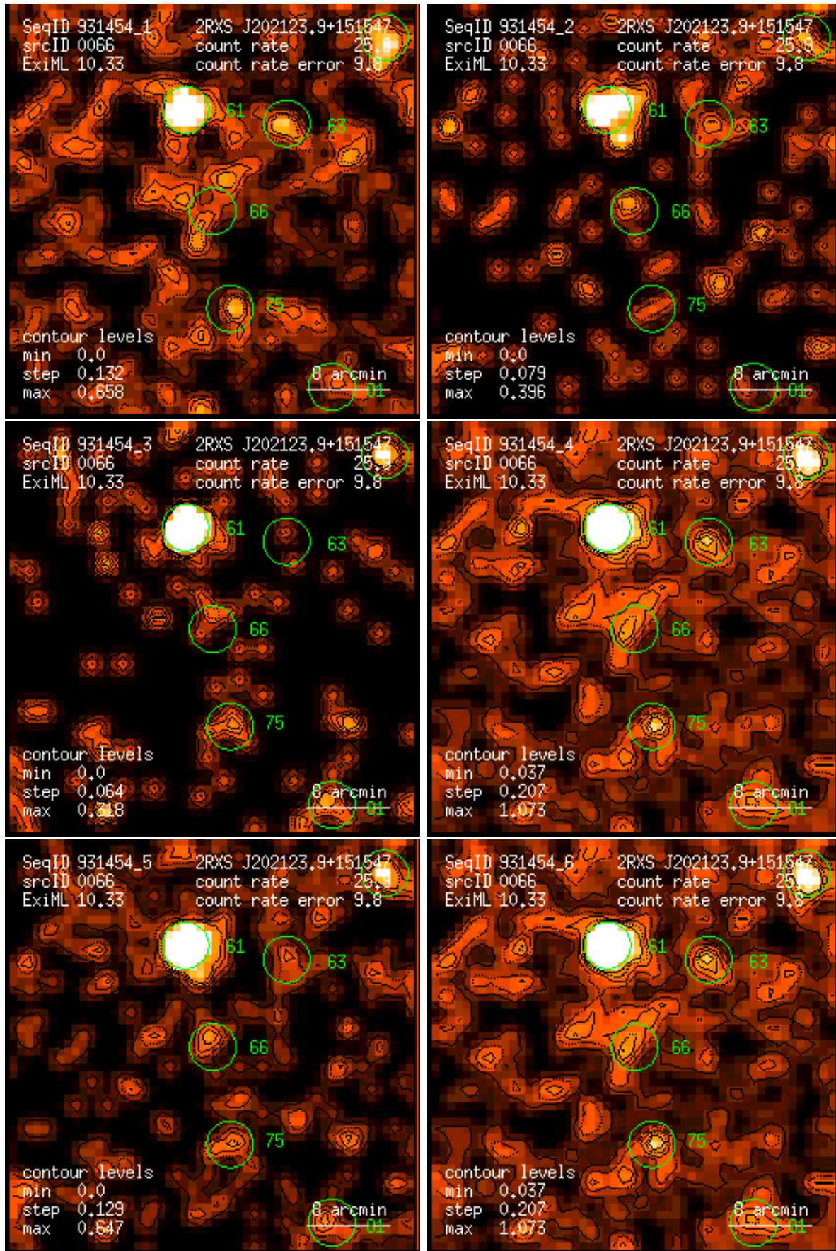
Figure 66: RASS 931454: detection 0066: band rate images, Gaussian filter: (1) PSPC channels 11 – 41, (2) 52 – 90, (3) 91 – 201, (4) 11 – 235, (5) 52 – 201, (6) 11 – 201. Broad band rates in counts/ks. Band rate contour levels in counts/ks/arcmin 2 .
