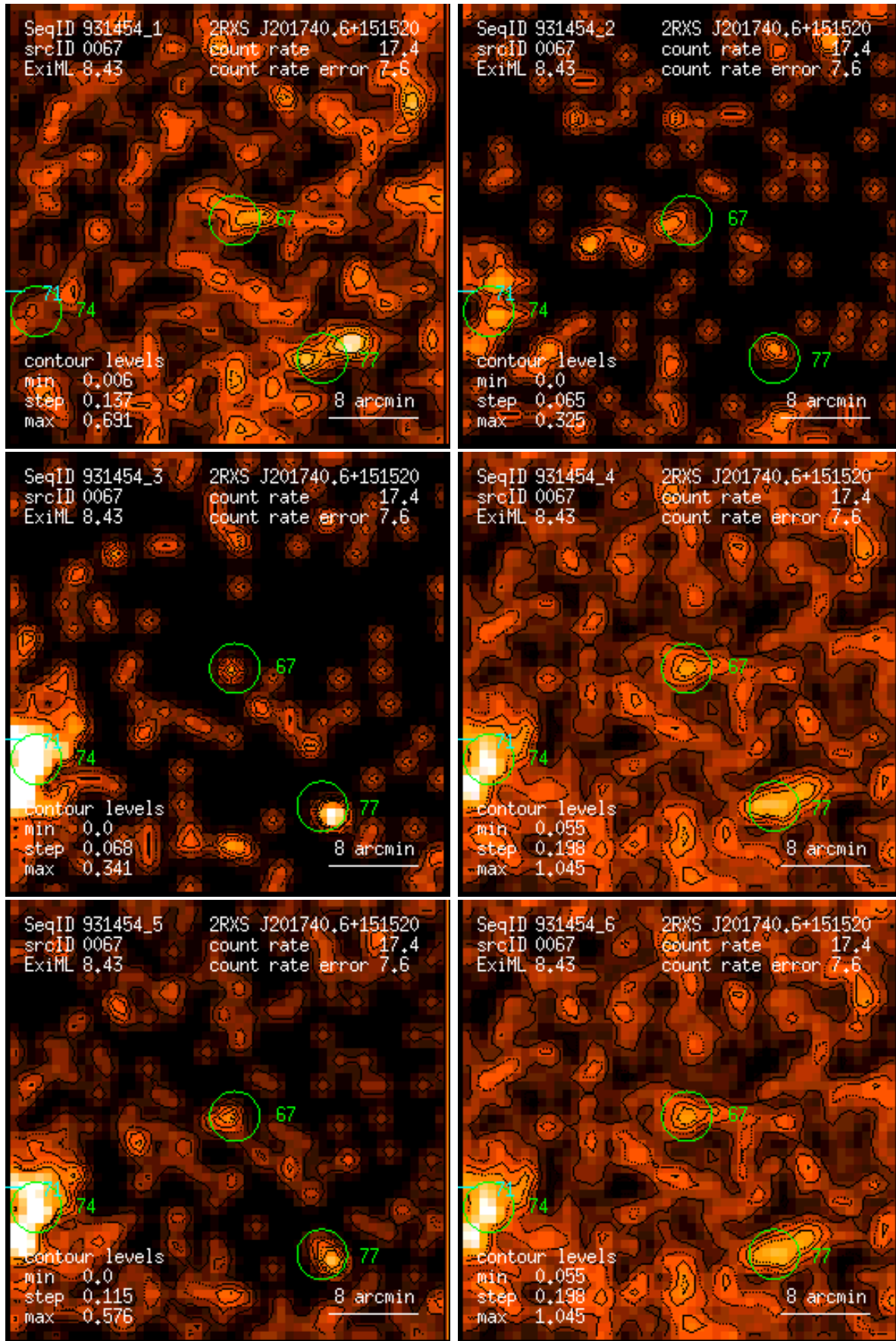
Figure 67: RASS 931454: detection 0067: band rate images, Gaussian filter: (1) PSPC channels 11 – 41, (2) 52 – 90, (3) 91 – 201, (4) 11 – 235, (5) 52 – 201, (6) 11 – 201. Broad band rates in counts/ks. Band rate contour levels in counts/ks/arcmin 2 .
