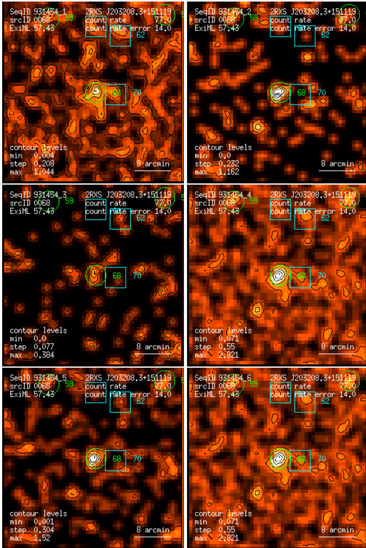
Figure 68: RASS 931454: detection 0068: band rate images, Gaussian filter: (1) PSPC channels 11 – 41, (2) 52 – 90, (3) 91 – 201, (4) 11 – 235, (5) 52 – 201, (6) 11 – 201. Broad band rates in counts/ks. Band rate contour levels in counts/ks/arcmin 2 .
