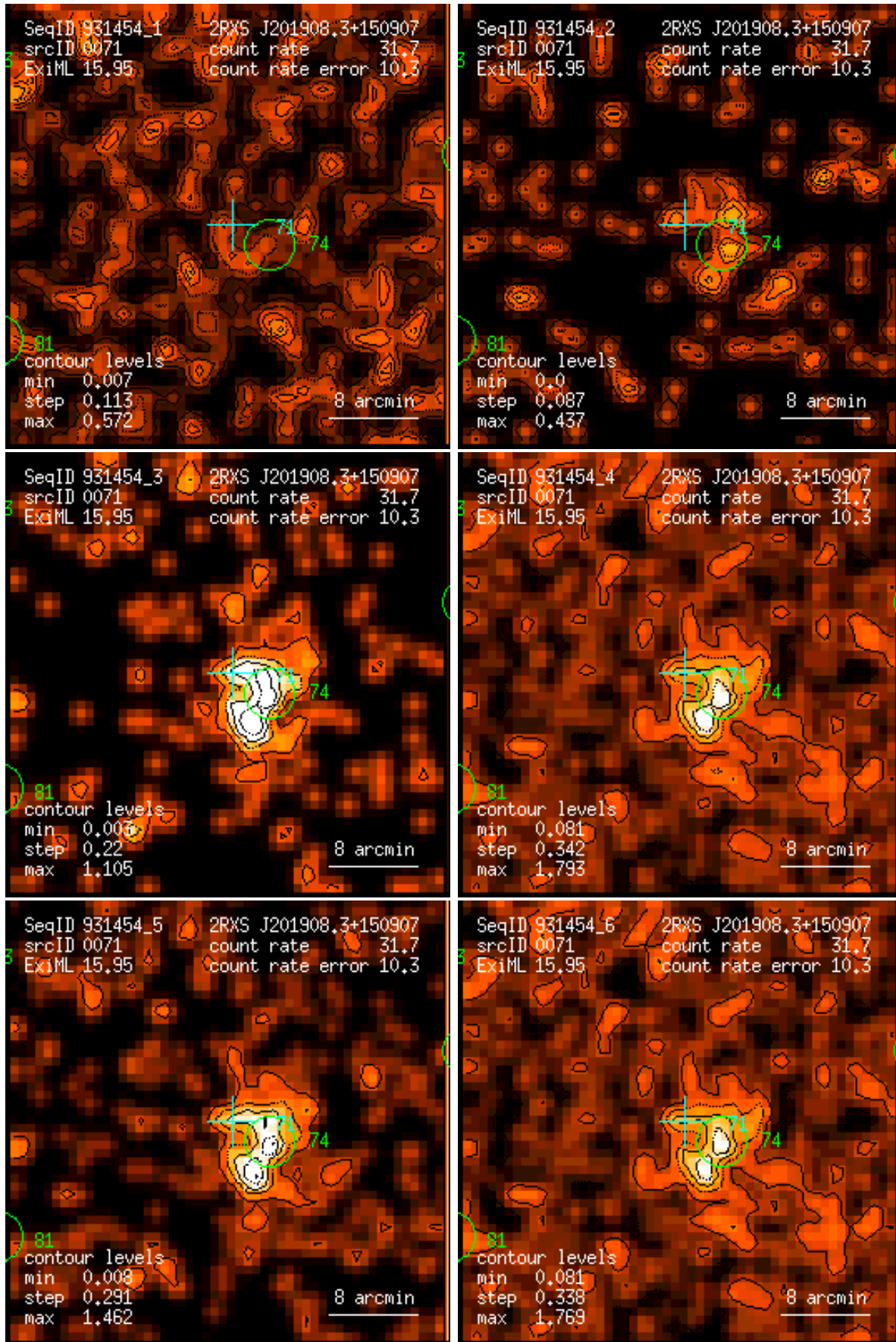
Figure 71: RASS 931454: detection 0071: band rate images, Gaussian filter: (1) PSPC channels 11 – 41, (2) 52 – 90, (3) 91 – 201, (4) 11 – 235, (5) 52 – 201, (6) 11 – 201. Broad band rates in counts/ks. Band rate contour levels in counts/ks/arcmin 2 .
