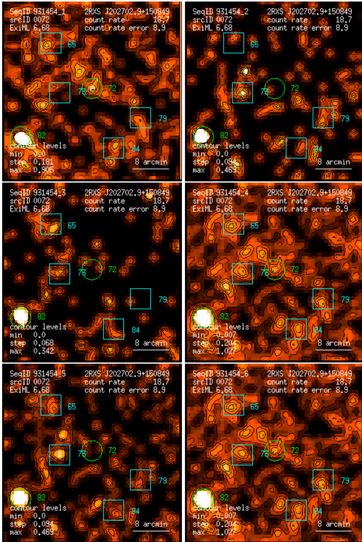
Figure 72: RASS 931454: detection 0072: band rate images, Gaussian filter: (1) PSPC channels 11 – 41, (2) 52 – 90, (3) 91 – 201, (4) 11 – 235, (5) 52 – 201, (6) 11 – 201. Broad band rates in counts/ks. Band rate contour levels in counts/ks/arcmin 2 .
