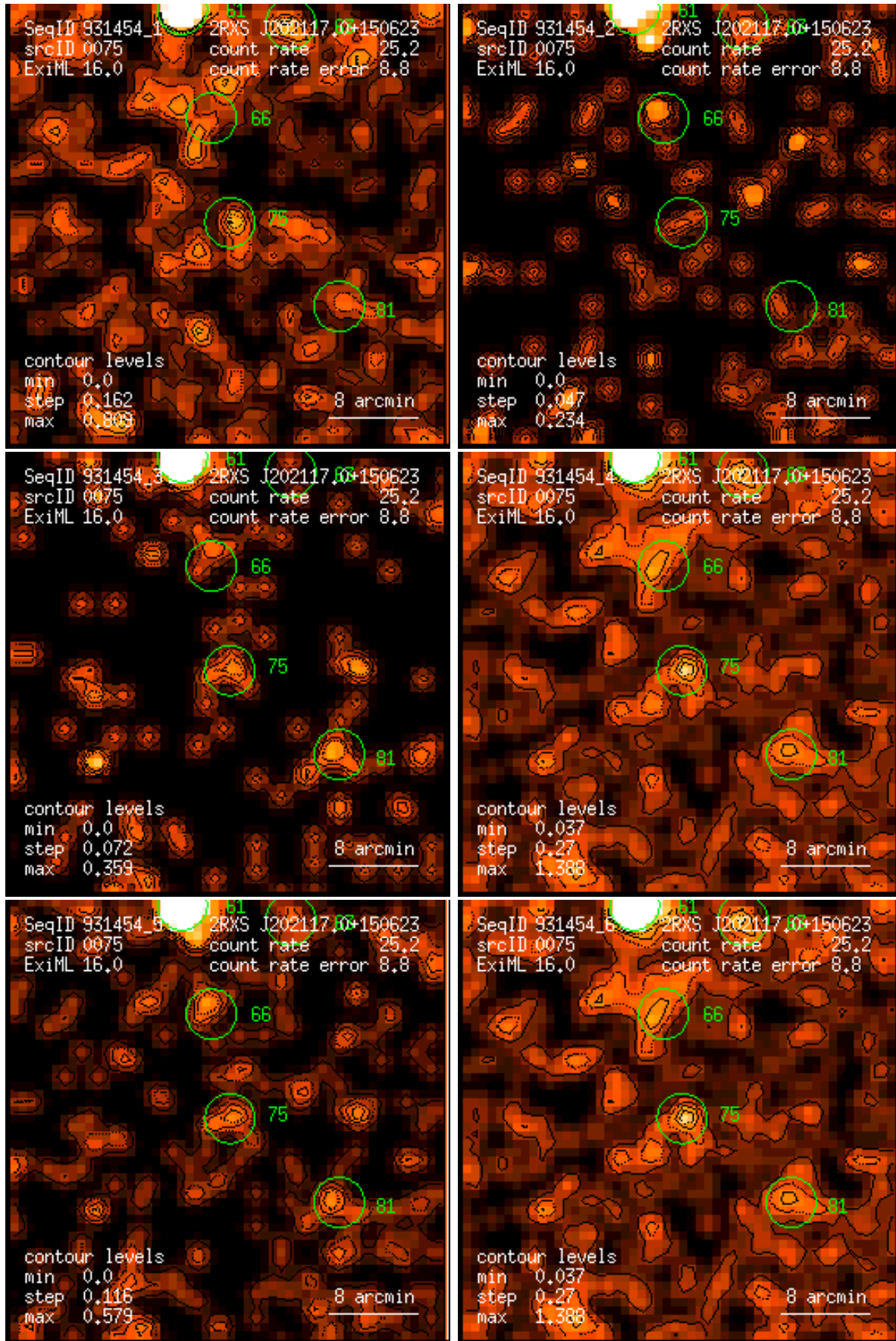
Figure 75: RASS 931454: detection 0075: band rate images, Gaussian filter: (1) PSPC channels 11 – 41, (2) 52 – 90, (3) 91 – 201, (4) 11 – 235, (5) 52 – 201, (6) 11 – 201. Broad band rates in counts/ks. Band rate contour levels in counts/ks/arcmin 2 .
