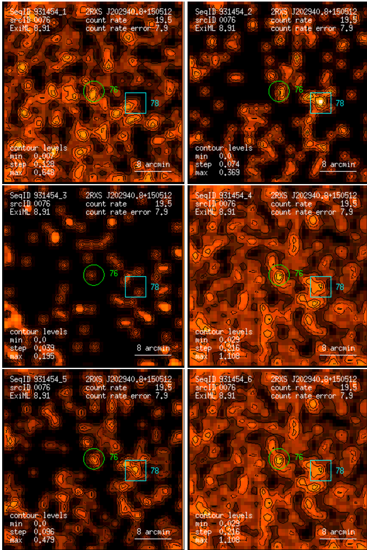
Figure 76: RASS 931454: detection 0076: band rate images, Gaussian filter: (1) PSPC channels 11 – 41, (2) 52 – 90, (3) 91 – 201, (4) 11 – 235, (5) 52 – 201, (6) 11 – 201. Broad band rates in counts/ks. Band rate contour levels in counts/ks/arcmin 2 .
