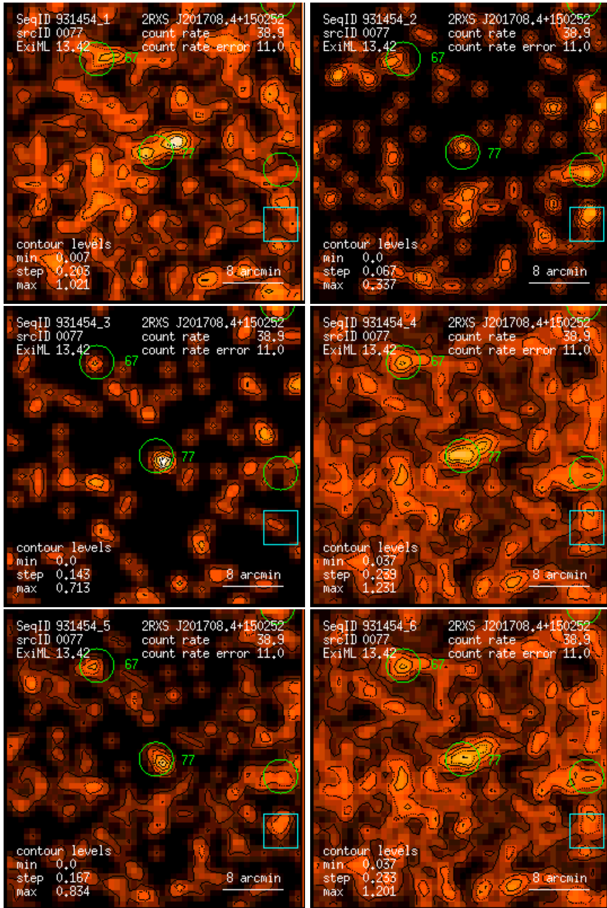
Figure 77: RASS 931454: detection 0077: band rate images, Gaussian filter: (1) PSPC channels 11 – 41, (2) 52 – 90, (3) 91 – 201, (4) 11 – 235, (5) 52 – 201, (6) 11 – 201. Broad band rates in counts/ks. Band rate contour levels in counts/ks/arcmin 2 .
