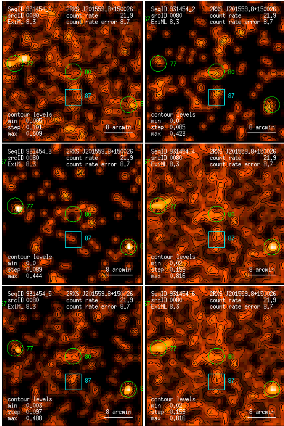
Figure 80: RASS 931454: detection 0080: band rate images, Gaussian filter: (1) PSPC channels 11 – 41, (2) 52 – 90, (3) 91 – 201, (4) 11 – 235, (5) 52 – 201, (6) 11 – 201. Broad band rates in counts/ks. Band rate contour levels in counts/ks/arcmin 2 .
