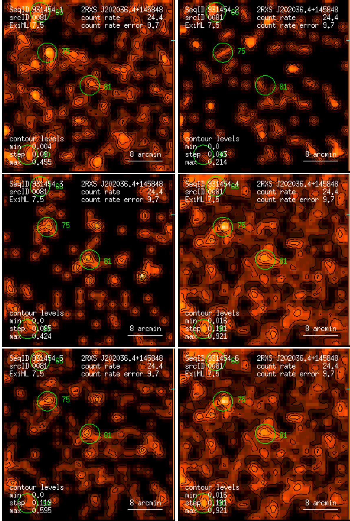
Figure 81: RASS 931454: detection 0081: band rate images, Gaussian filter: (1) PSPC channels 11 – 41, (2) 52 – 90, (3) 91 – 201, (4) 11 – 235, (5) 52 – 201, (6) 11 – 201. Broad band rates in counts/ks. Band rate contour levels in counts/ks/arcmin 2 .
