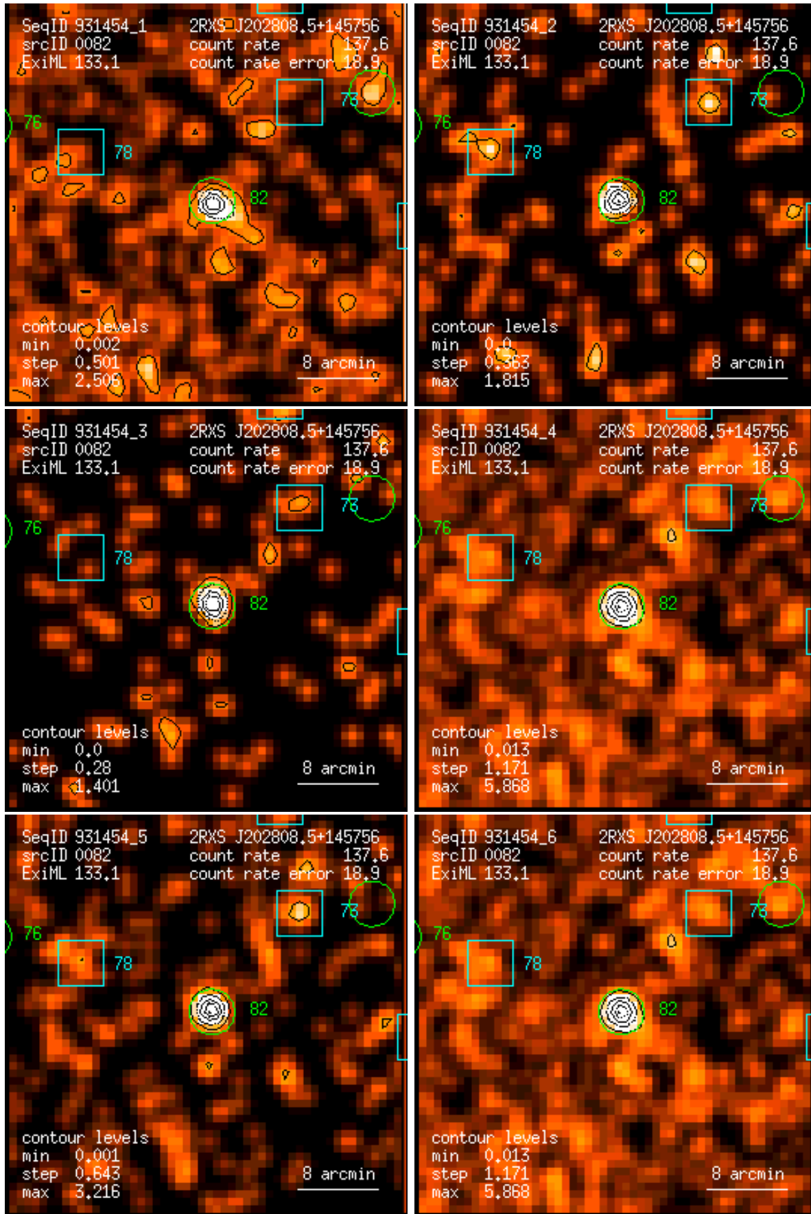
Figure 82: RASS 931454: detection 0082: band rate images, Gaussian filter: (1) PSPC channels 11 – 41, (2) 52 – 90, (3) 91 – 201, (4) 11 – 235, (5) 52 – 201, (6) 11 – 201. Broad band rates in counts/ks. Band rate contour levels in counts/ks/arcmin 2 .
