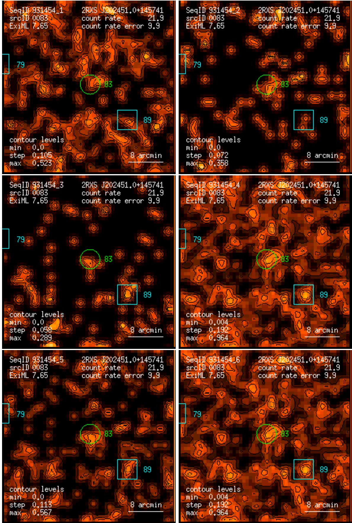
Figure 83: RASS 931454: detection 0083: band rate images, Gaussian filter: (1) PSPC channels 11 – 41, (2) 52 – 90, (3) 91 – 201, (4) 11 – 235, (5) 52 – 201, (6) 11 – 201. Broad band rates in counts/ks. Band rate contour levels in counts/ks/arcmin 2 .
