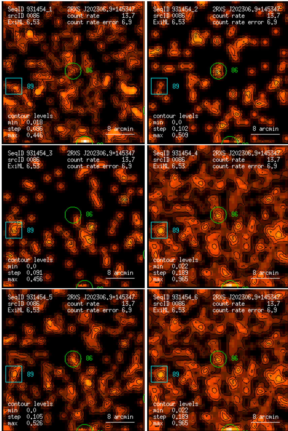
Figure 86: RASS 931454: detection 0086: band rate images, Gaussian filter: (1) PSPC channels 11 – 41, (2) 52 – 90, (3) 91 – 201, (4) 11 – 235, (5) 52 – 201, (6) 11 – 201. Broad band rates in counts/ks. Band rate contour levels in counts/ks/arcmin 2 .
