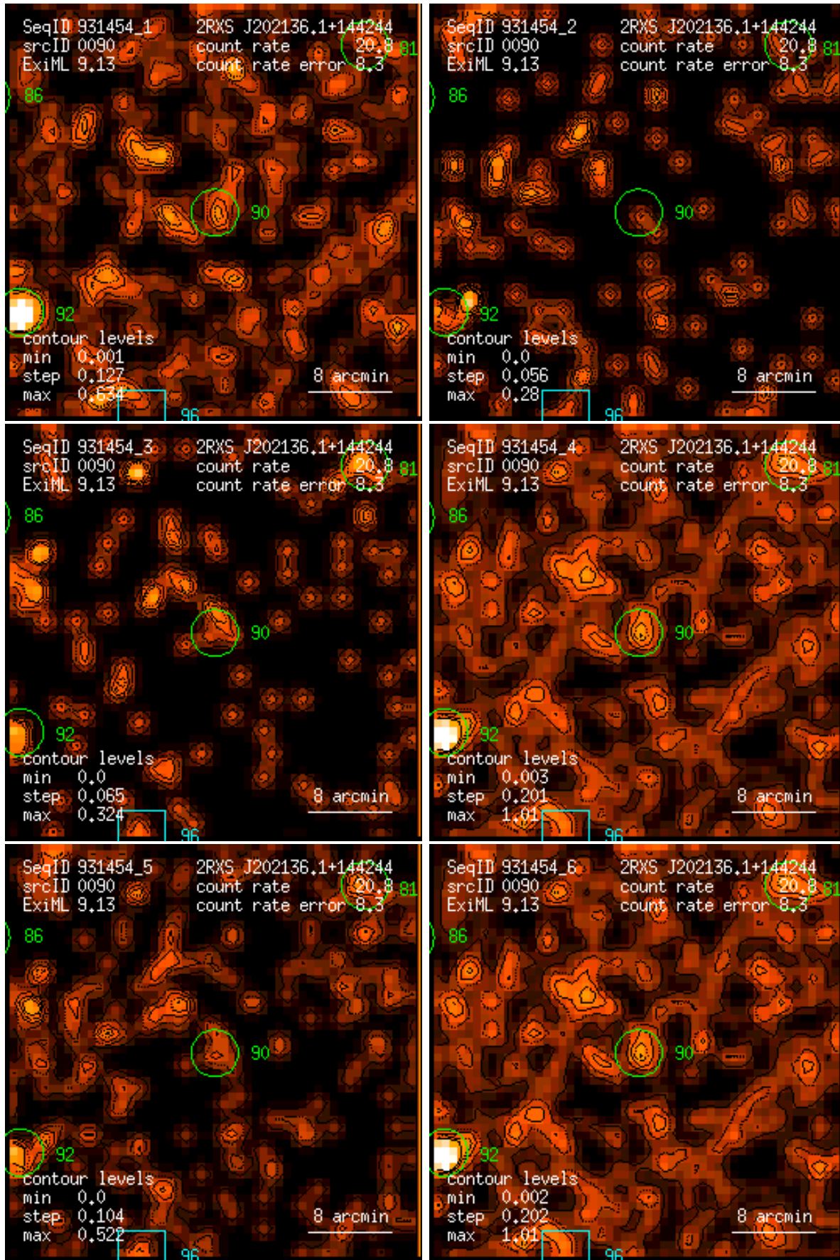
Figure 90: RASS 931454: detection 0090: band rate images, Gaussian filter: (1) PSPC channels 11 – 41, (2) 52 – 90, (3) 91 – 201, (4) 11 – 235, (5) 52 – 201, (6) 11 – 201. Broad band rates in counts/ks. Band rate contour levels in counts/ks/arcmin 2 .
