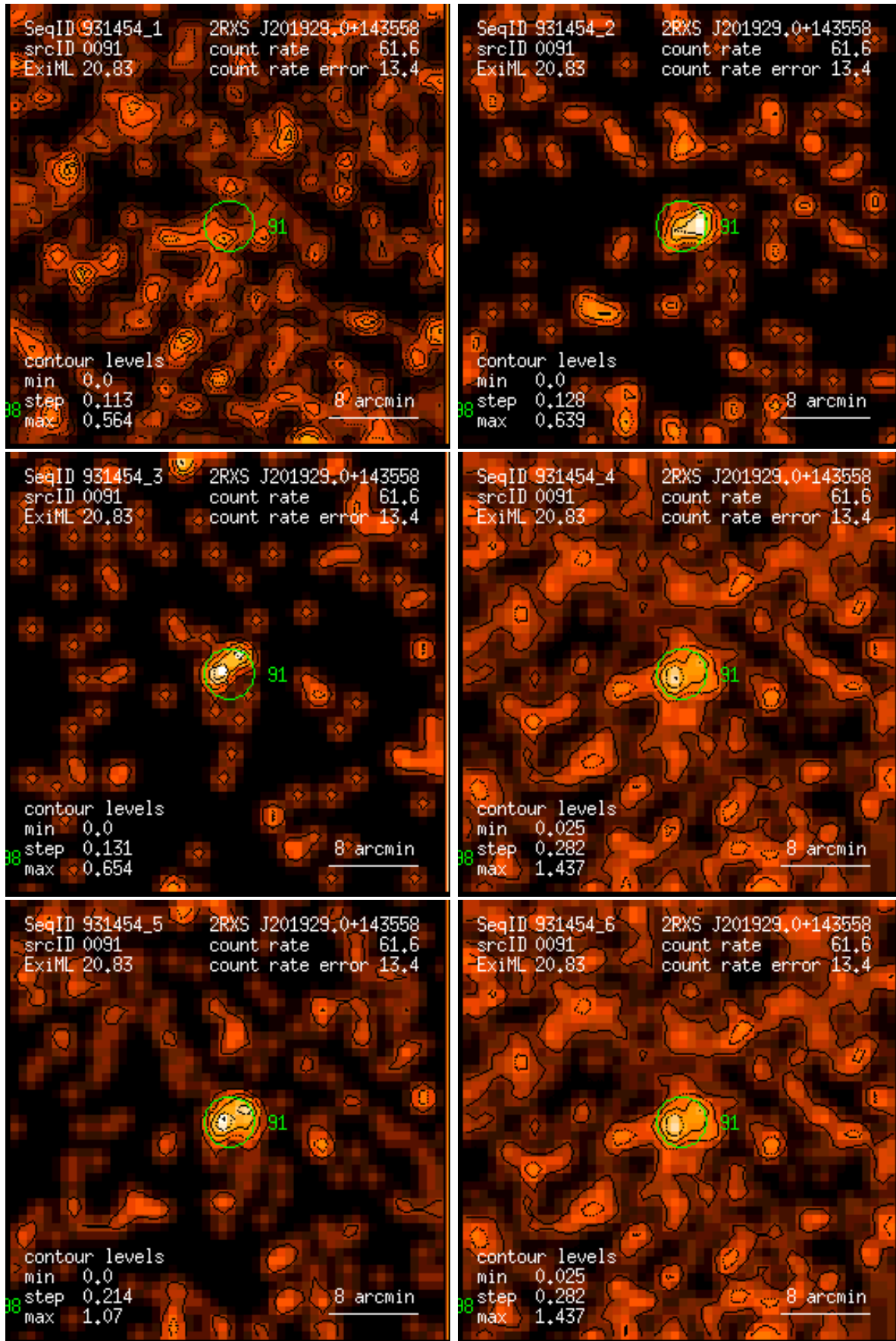
Figure 91: RASS 931454: detection 0091: band rate images, Gaussian filter: (1) PSPC channels 11 – 41, (2) 52 – 90, (3) 91 – 201, (4) 11 – 235, (5) 52 – 201, (6) 11 – 201. Broad band rates in counts/ks. Band rate contour levels in counts/ks/arcmin 2 .
