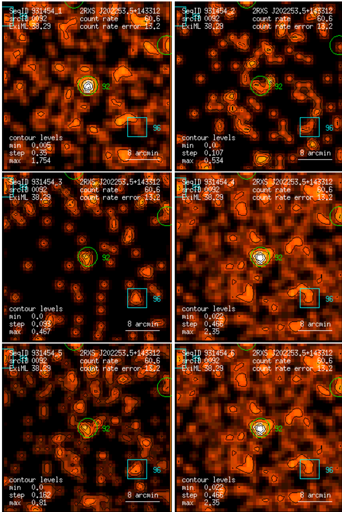
Figure 92: RASS 931454: detection 0092: band rate images, Gaussian filter: (1) PSPC channels 11 – 41, (2) 52 – 90, (3) 91 – 201, (4) 11 – 235, (5) 52 – 201, (6) 11 – 201. Broad band rates in counts/ks. Band rate contour levels in counts/ks/arcmin 2 .
