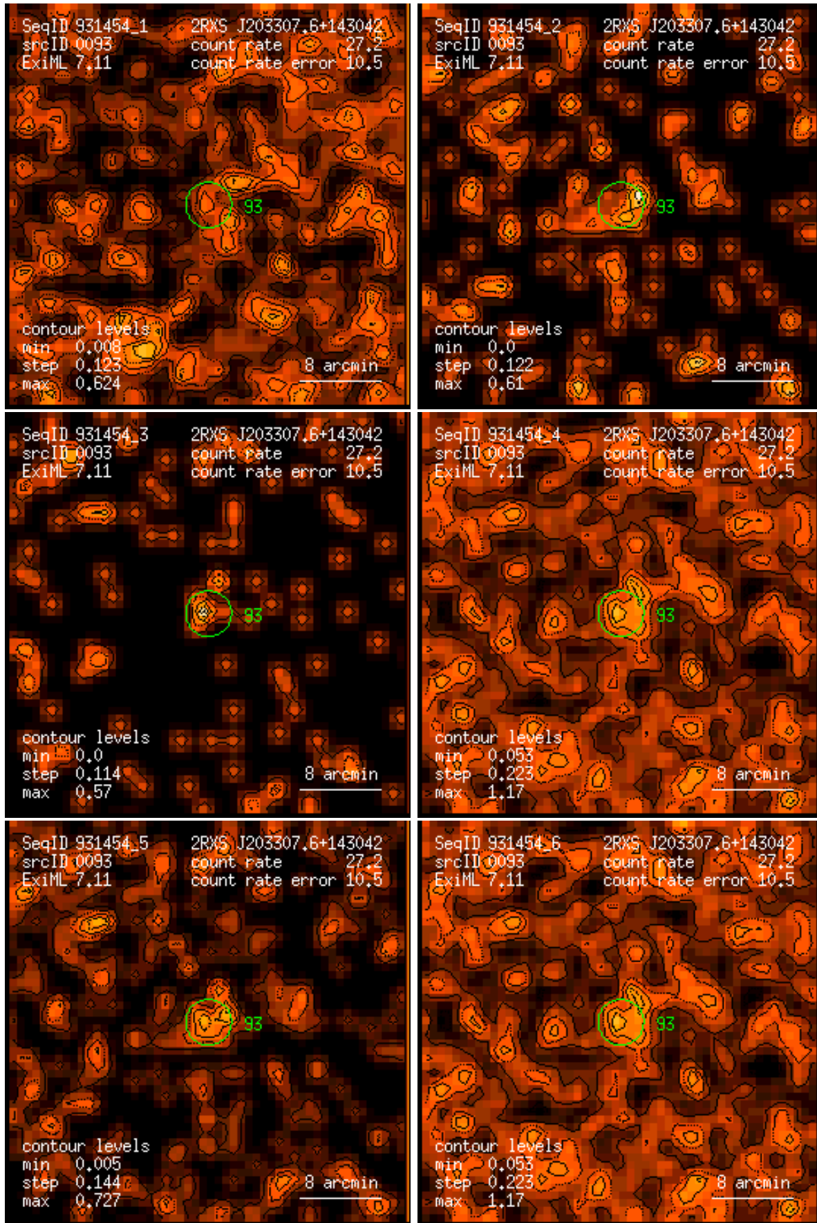
Figure 93: RASS 931454: detection 0093: band rate images, Gaussian filter: (1) PSPC channels 11 – 41, (2) 52 – 90, (3) 91 – 201, (4) 11 – 235, (5) 52 – 201, (6) 11 – 201. Broad band rates in counts/ks. Band rate contour levels in counts/ks/arcmin 2 .
