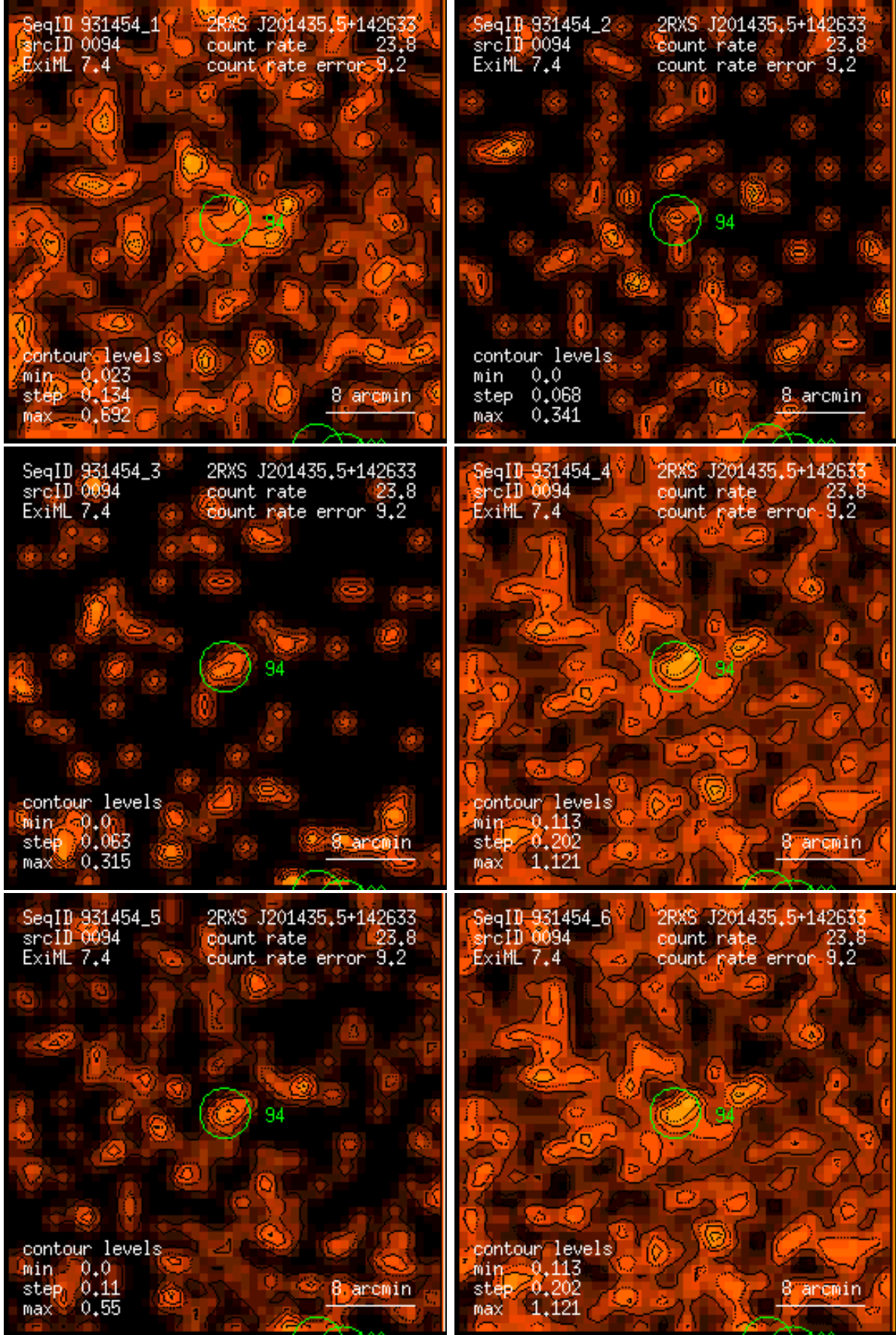
Figure 94: RASS 931454: detection 0094: band rate images, Gaussian filter: (1) PSPC channels 11 – 41, (2) 52 – 90, (3) 91 – 201, (4) 11 – 235, (5) 52 – 201, (6) 11 – 201. Broad band rates in counts/ks. Band rate contour levels in counts/ks/arcmin 2 .
