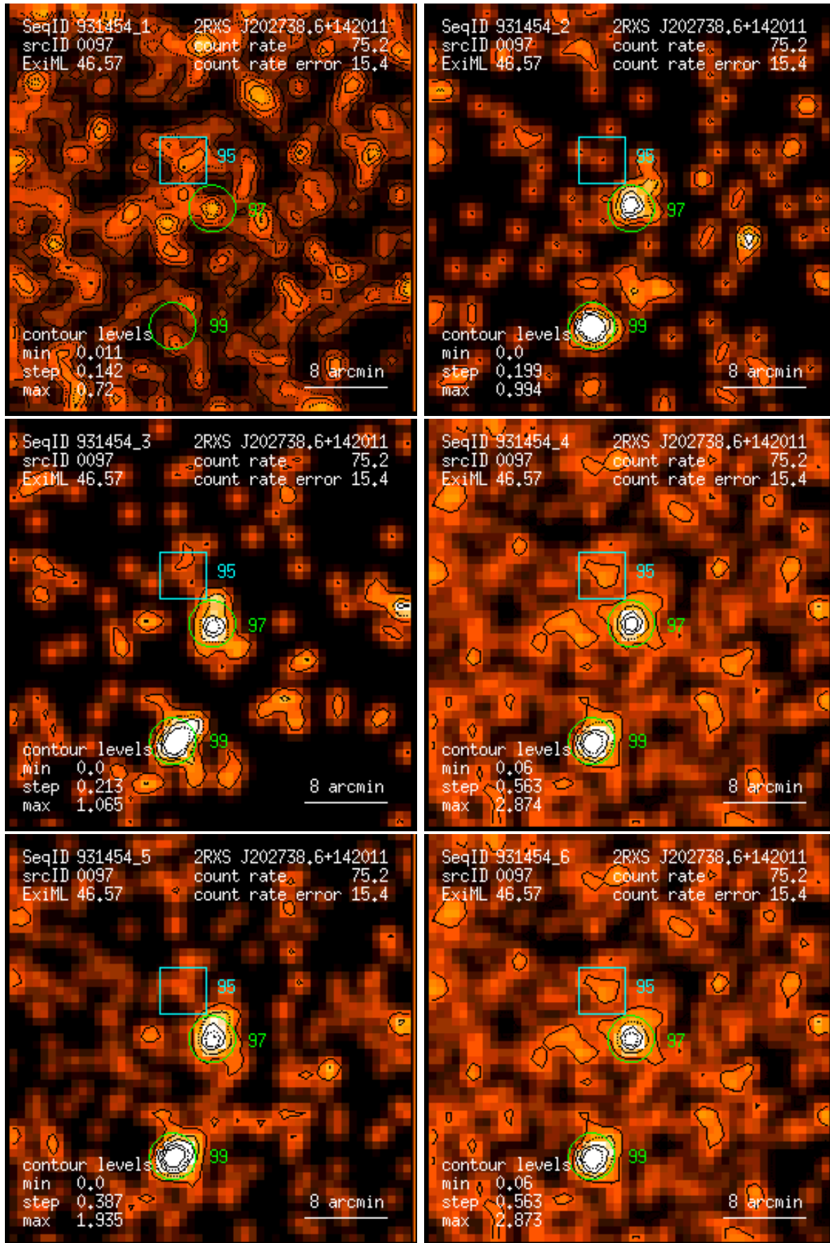
Figure 97: RASS 931454: detection 0097: band rate images, Gaussian filter: (1) PSPC channels 11 – 41, (2) 52 – 90, (3) 91 – 201, (4) 11 – 235, (5) 52 – 201, (6) 11 – 201. Broad band rates in counts/ks. Band rate contour levels in counts/ks/arcmin 2 .
