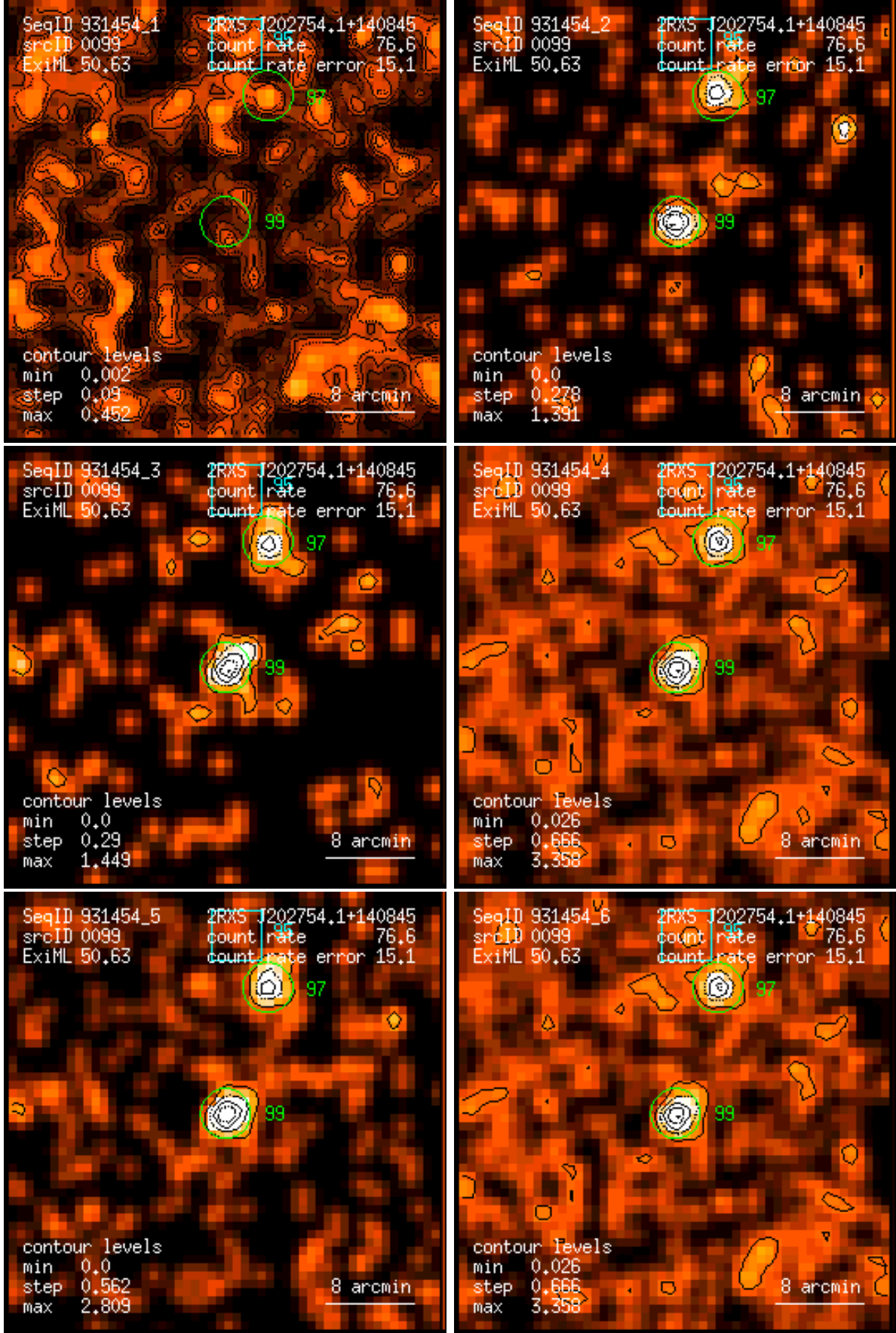
Figure 99: RASS 931454: detection 0099: band rate images, Gaussian filter: (1) PSPC channels 11 – 41, (2) 52 – 90, (3) 91 – 201, (4) 11 – 235, (5) 52 – 201, (6) 11 – 201. Broad band rates in counts/ks. Band rate contour levels in counts/ks/arcmin 2 .
