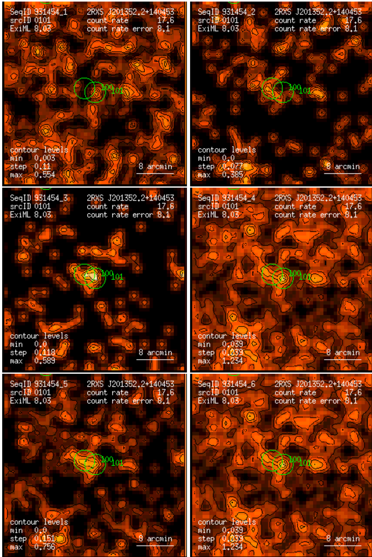
Figure 101: RASS 931454: detection 0101: band rate images, Gaussian filter: (1) PSPC channels 11 – 41, (2) 52 – 90, (3) 91 – 201, (4) 11 – 235, (5) 52 – 201, (6) 11 – 201. Broad band rates in counts/ks. Band rate contour levels in counts/ks/arcmin 2 .
