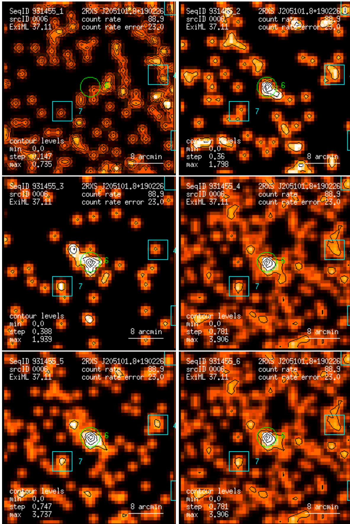
Figure 6: RASS 931455: detection 0006: band rate images, Gaussian filter: (1) PSPC channels 11 – 41, (2) 52 – 90, (3) 91 – 201, (4) 11 – 235, (5) 52 – 201, (6) 11 – 201. Broad band rates in counts/ks. Band rate contour levels in counts/ks/arcmin 2 .
