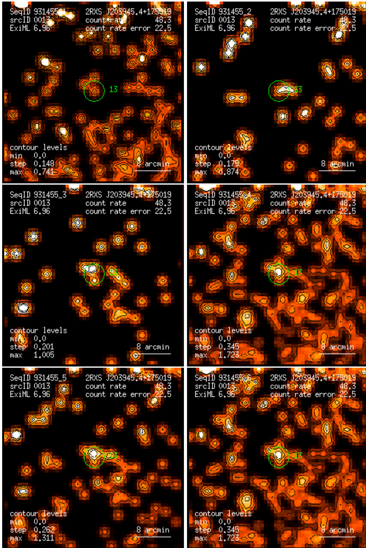
Figure 13: RASS 931455: detection 0013: band rate images, Gaussian filter: (1) PSPC channels 11 – 41, (2) 52 – 90, (3) 91 – 201, (4) 11 – 235, (5) 52 – 201, (6) 11 – 201. Broad band rates in counts/ks. Band rate contour levels in counts/ks/arcmin 2 .
