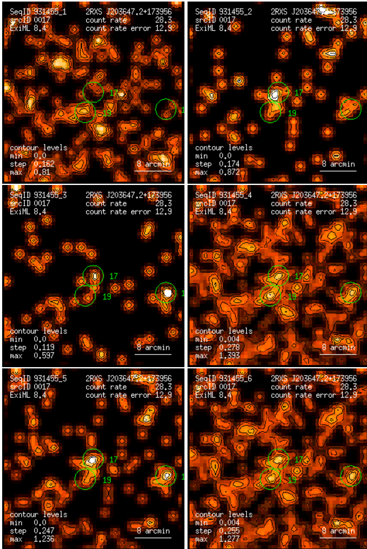
Figure 17: RASS 931455: detection 0017: band rate images, Gaussian filter: (1) PSPC channels 11 – 41, (2) 52 – 90, (3) 91 – 201, (4) 11 – 235, (5) 52 – 201, (6) 11 – 201. Broad band rates in counts/ks. Band rate contour levels in counts/ks/arcmin 2 .
