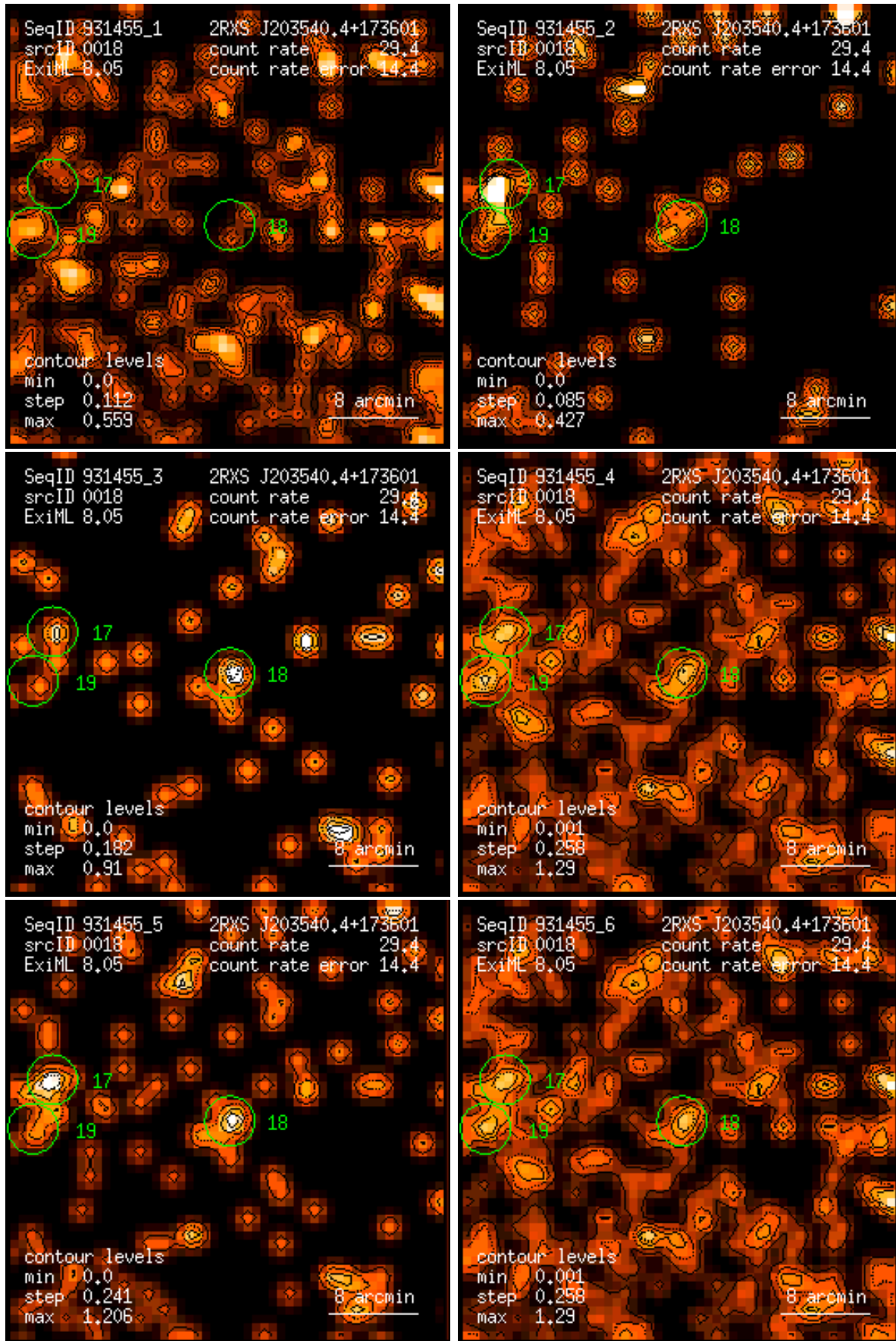
Figure 18: RASS 931455: detection 0018: band rate images, Gaussian filter: (1) PSPC channels 11 – 41, (2) 52 – 90, (3) 91 – 201, (4) 11 – 235, (5) 52 – 201, (6) 11 – 201. Broad band rates in counts/ks. Band rate contour levels in counts/ks/arcmin 2 .
