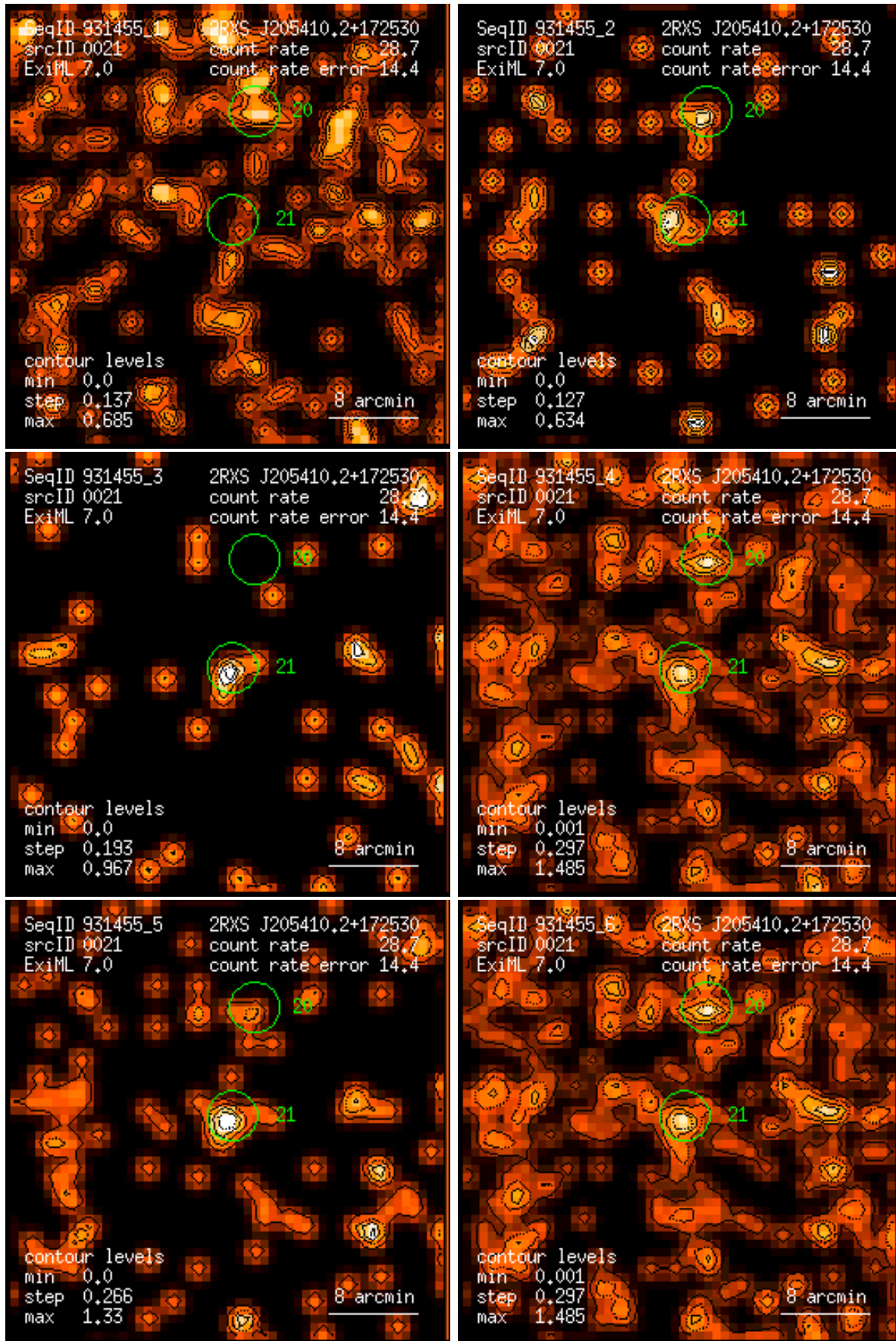
Figure 21: RASS 931455: detection 0021: band rate images, Gaussian filter: (1) PSPC channels 11 – 41, (2) 52 – 90, (3) 91 – 201, (4) 11 – 235, (5) 52 – 201, (6) 11 – 201. Broad band rates in counts/ks. Band rate contour levels in counts/ks/arcmin 2 .
