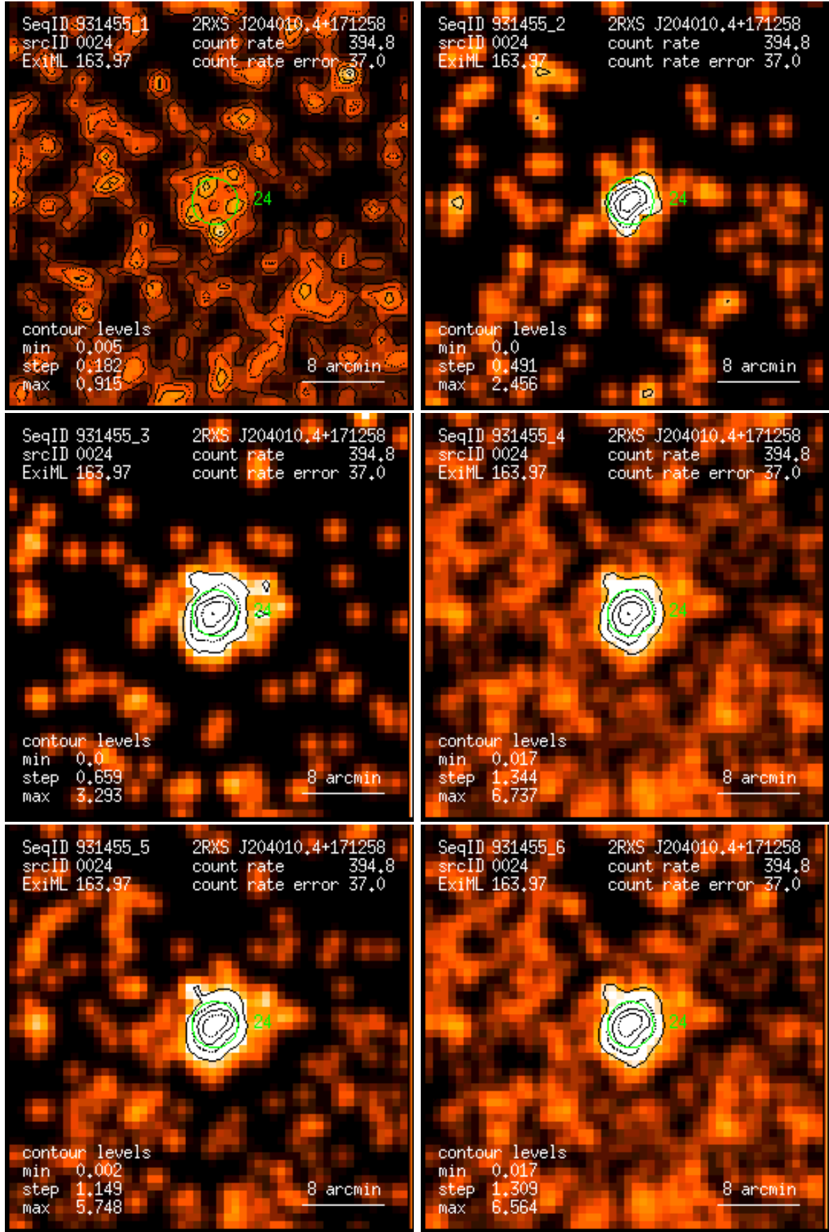
Figure 24: RASS 931455: detection 0024: band rate images, Gaussian filter: (1) PSPC channels 11 – 41, (2) 52 – 90, (3) 91 – 201, (4) 11 – 235, (5) 52 – 201, (6) 11 – 201. Broad band rates in counts/ks. Band rate contour levels in counts/ks/arcmin 2 .
